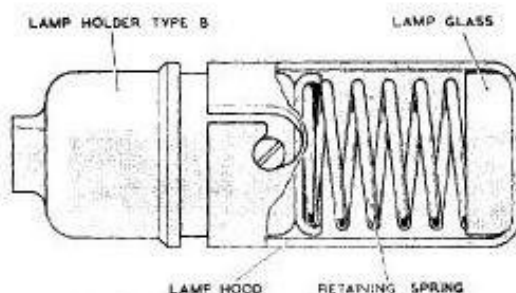
Fig. 1. de Havilland dash flood lamp
