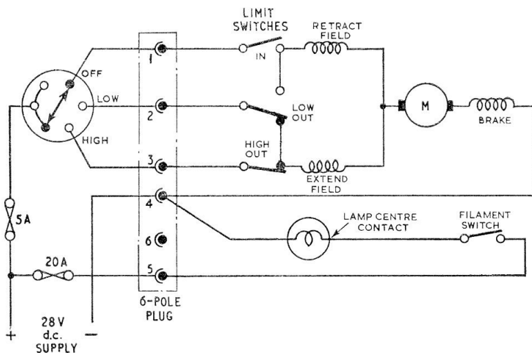
Fig. 3. Circuit diagram
