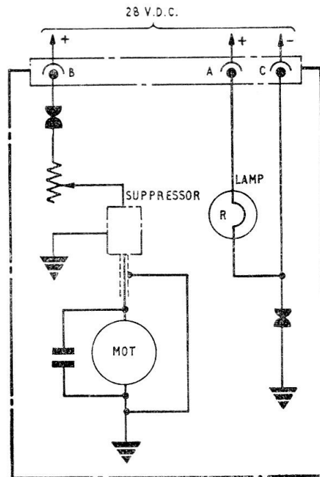
Fig. 1. Circuit diagram
