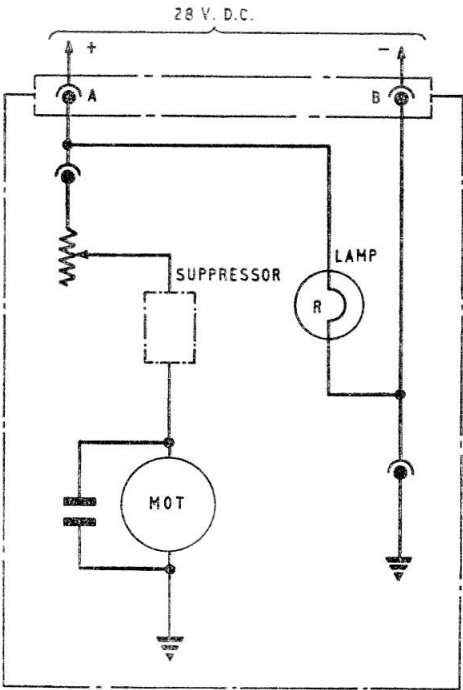
Fig. 1. Circuit diagram
