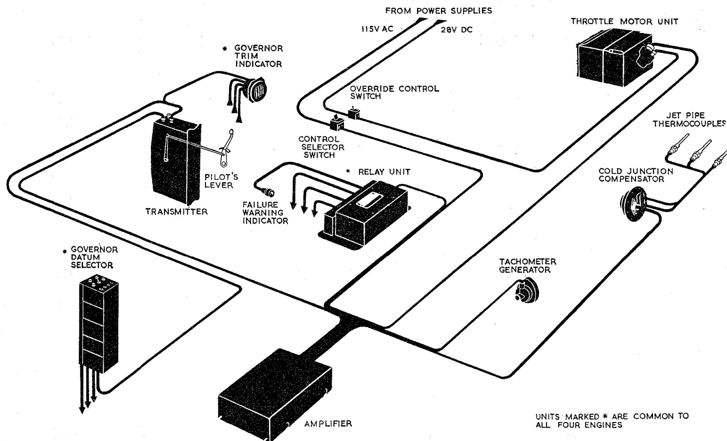
Fig. 1. Layout of B.A.P.3 system for one engine
