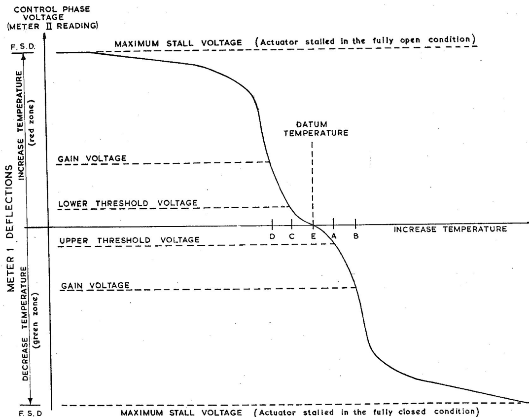
Fig. 5. Response diagram
