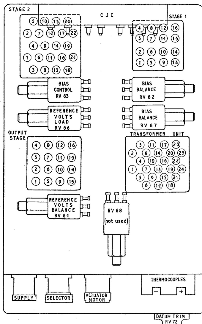
Fig. 7. Layout of amplifier, showing seal numbers
