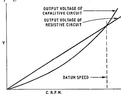
Fig. 4 Output voltages of datum selector unit
