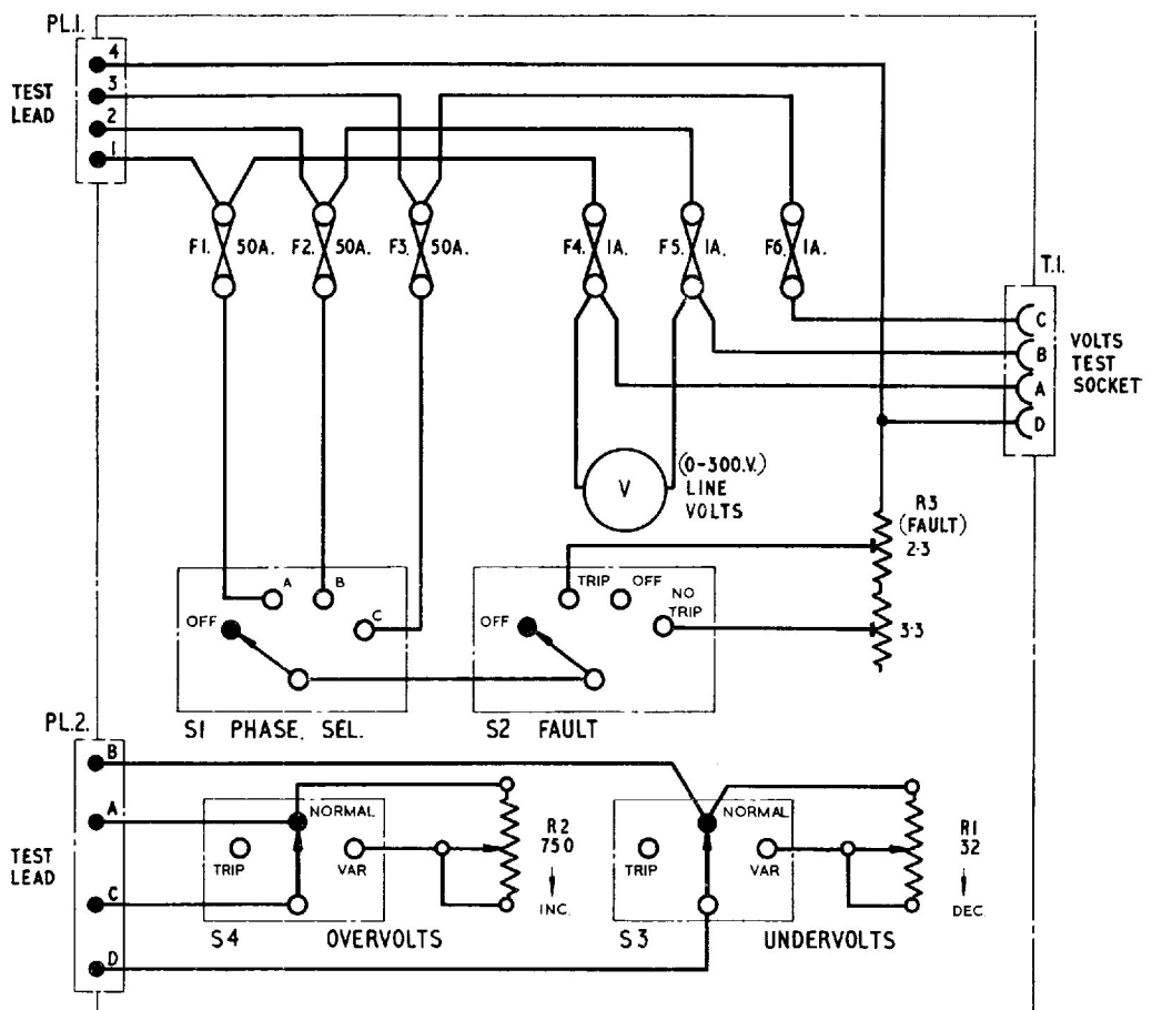
Fig. 3. Circuit diagram
