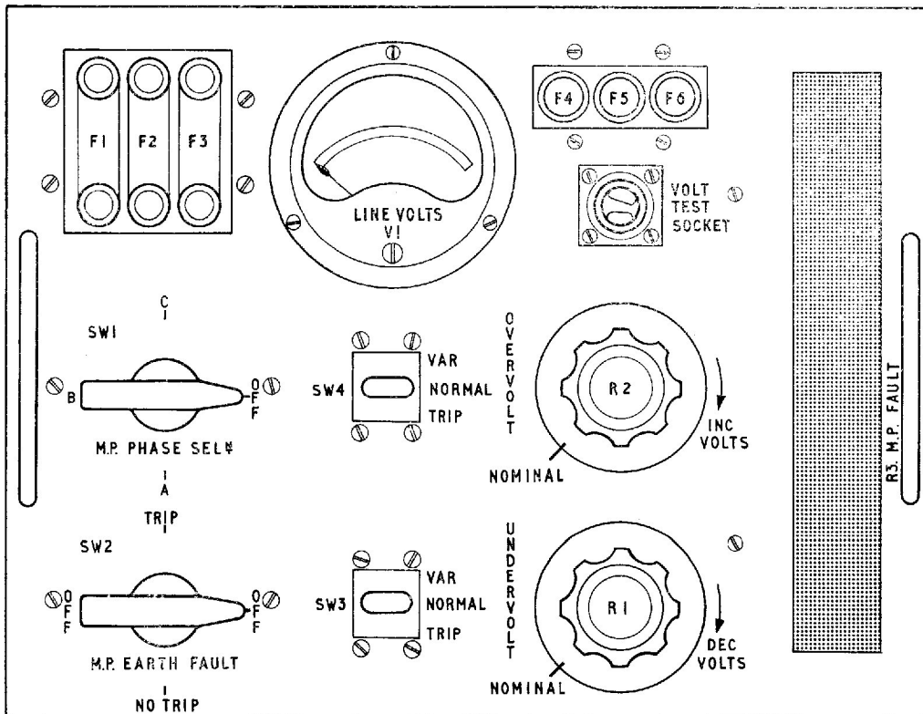
Fig. 2. Test panel
