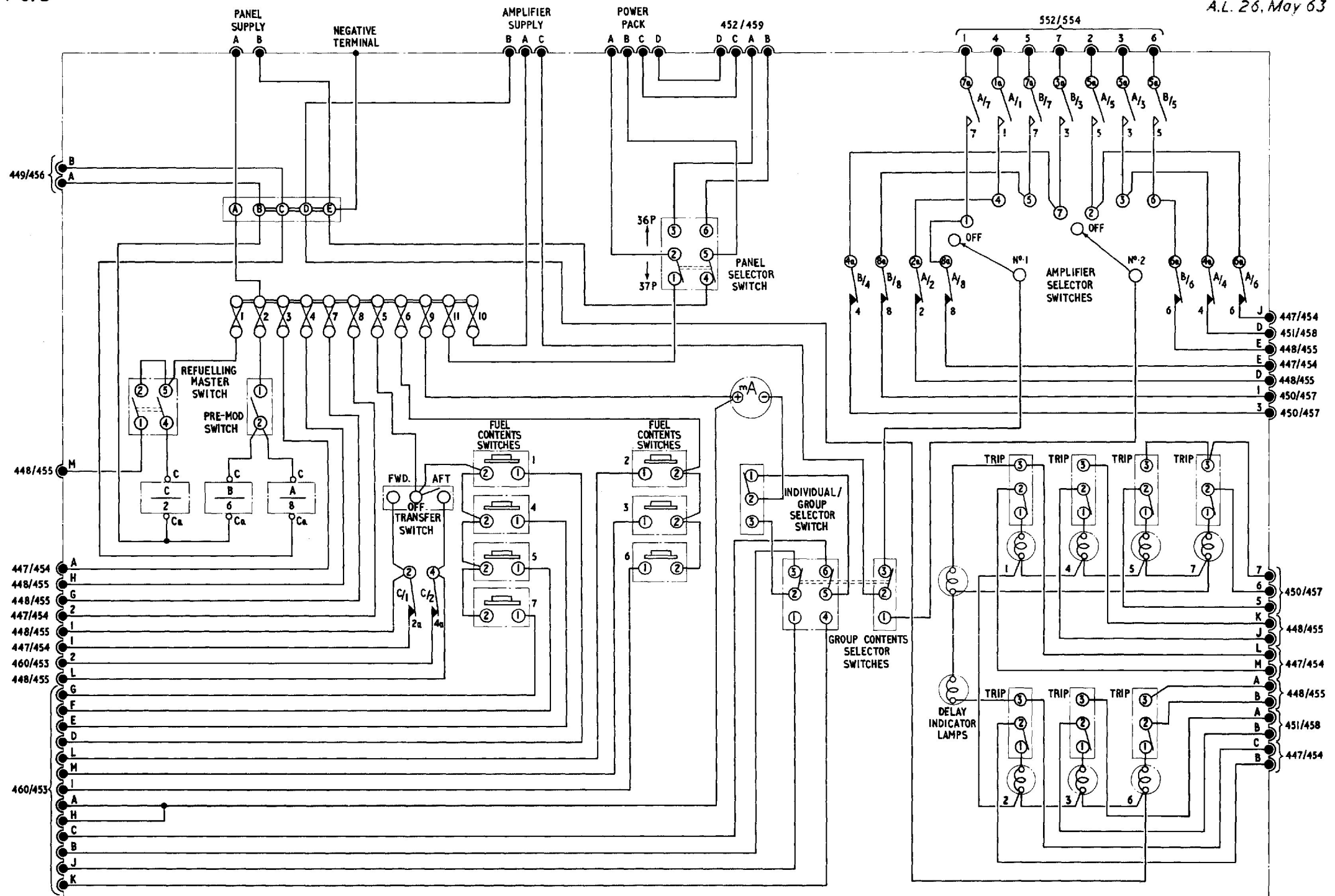
FIG.2 CIRCUIT DIAGRAM (TEST PANEL)
