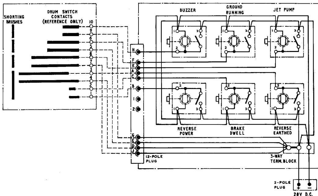
Fig. 2. Circuit diagram
