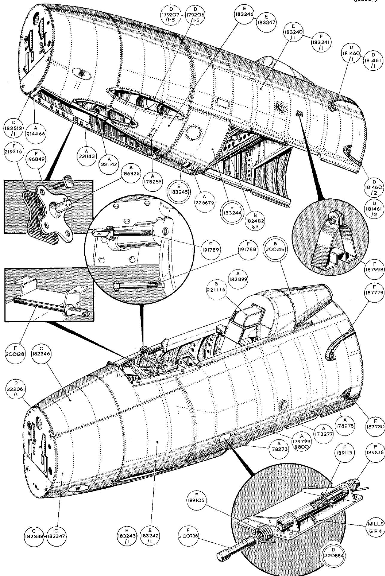
FRONT FUSELAGE
