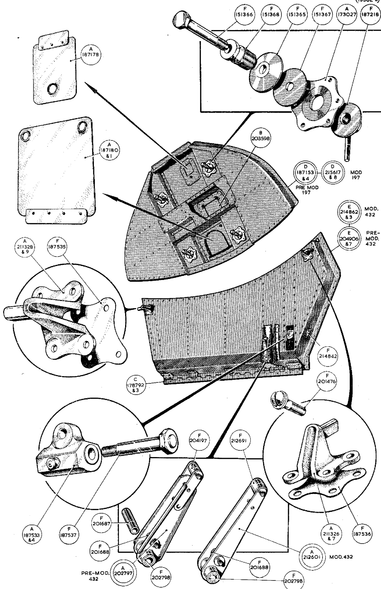
MAIN UNDERCARRIAGE
