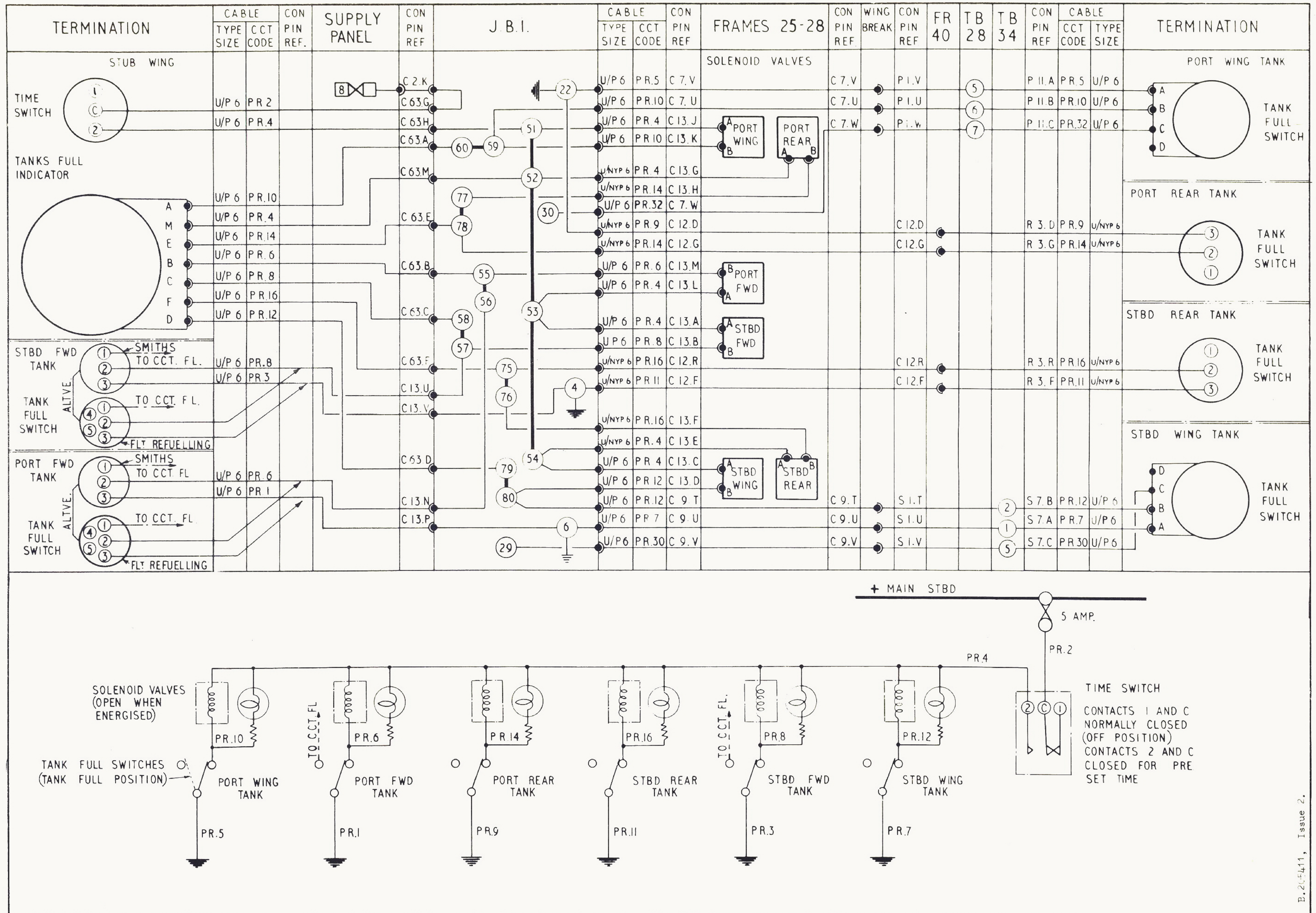
FIG. 2 PRESSURE RE-FUELLING
