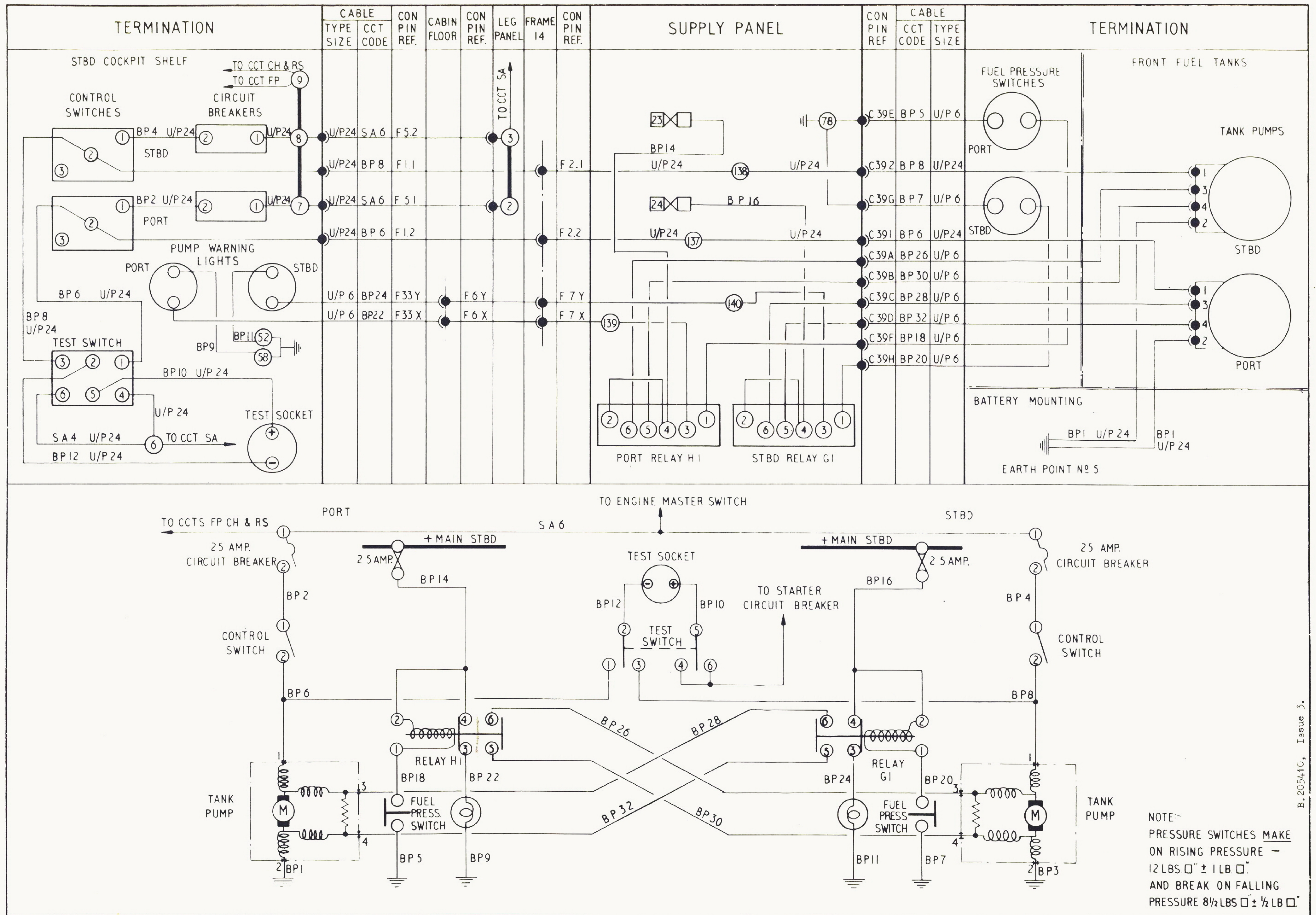
FIG. 1. TANK PUMPS RESTRICTED
