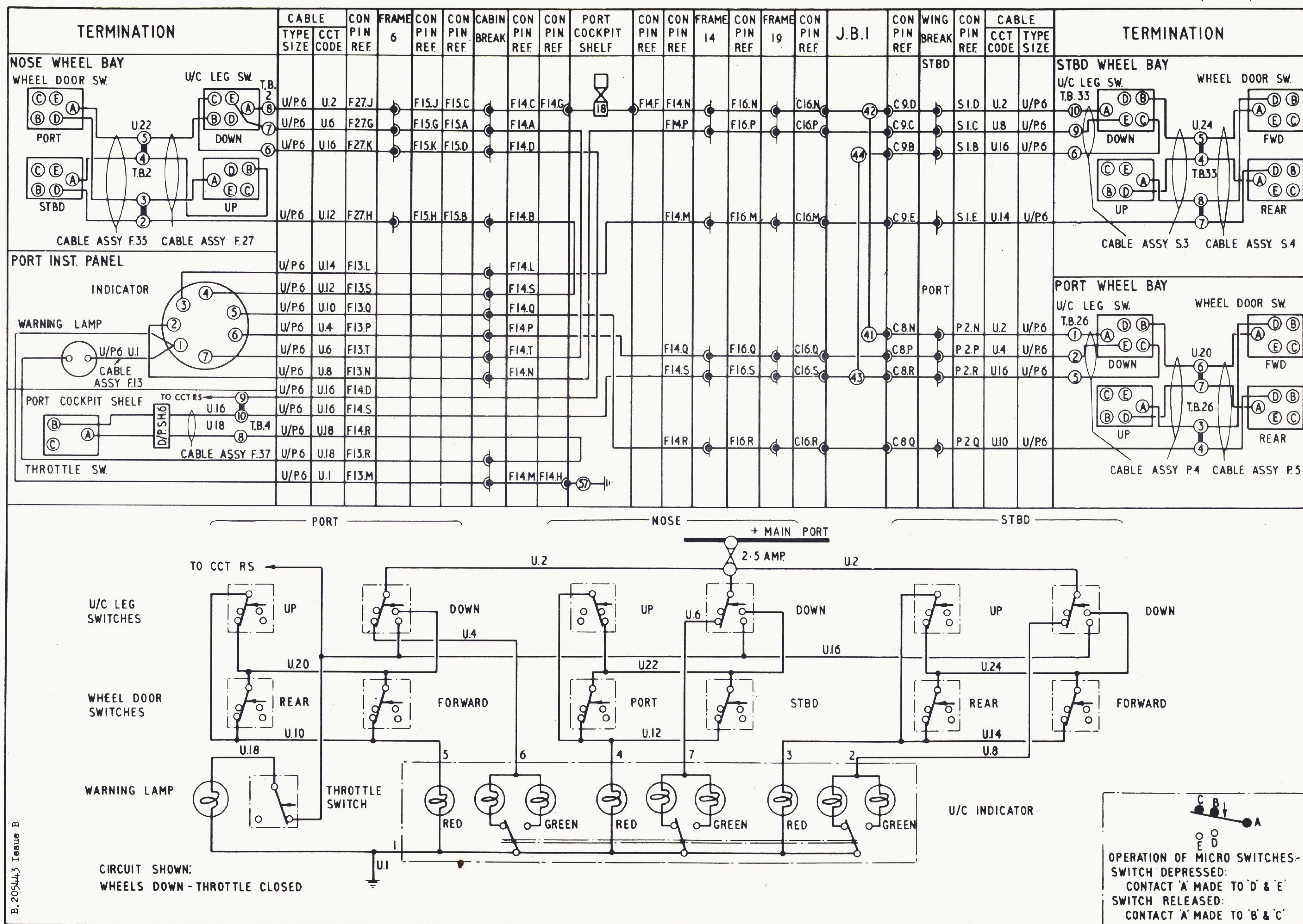
FIG. 1. ALIGHTING GEAR INDICATOR
