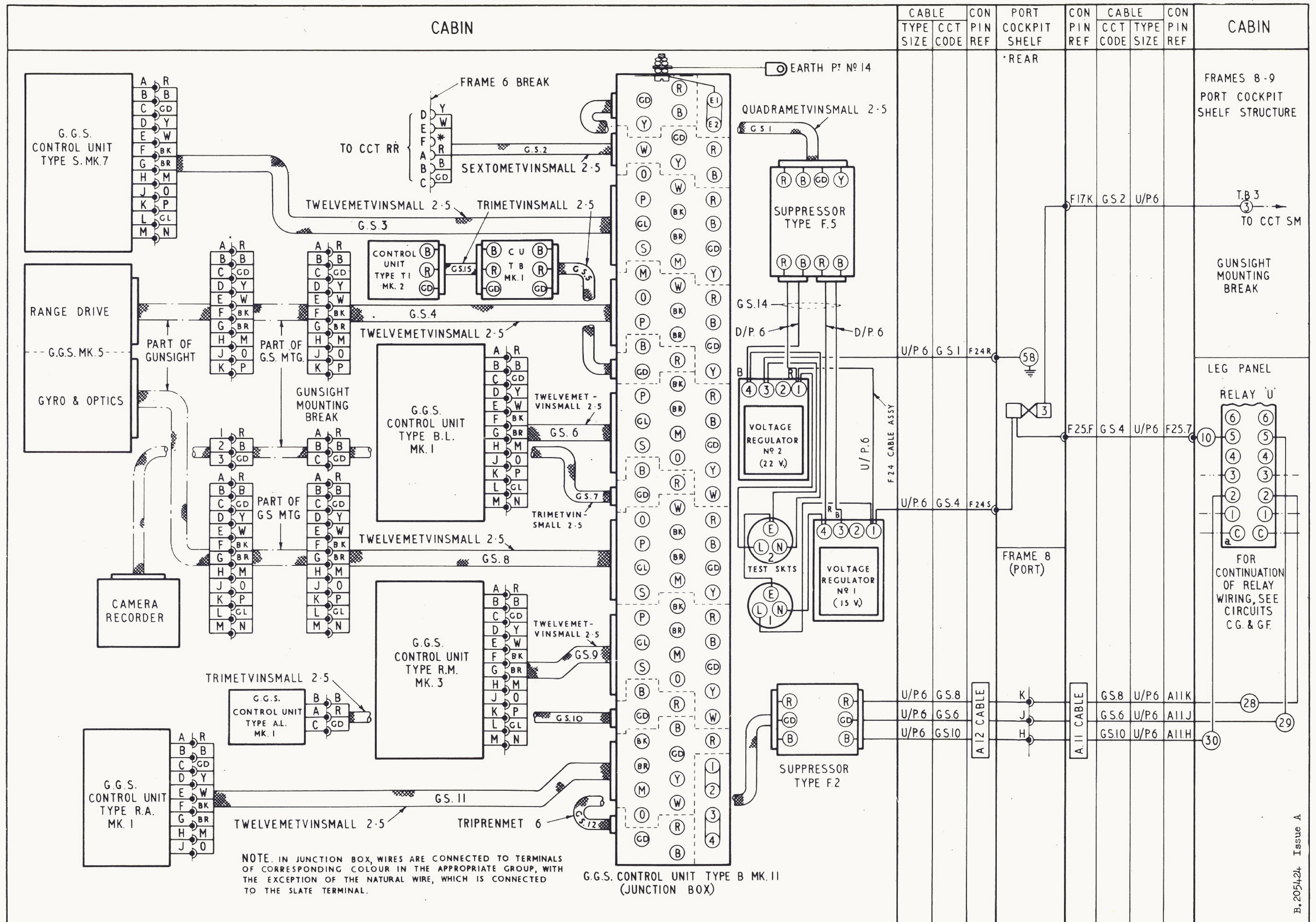
FIG.2 GYRO GUN-SIGHT AND CAMERA RECORDER (ROUTING)
