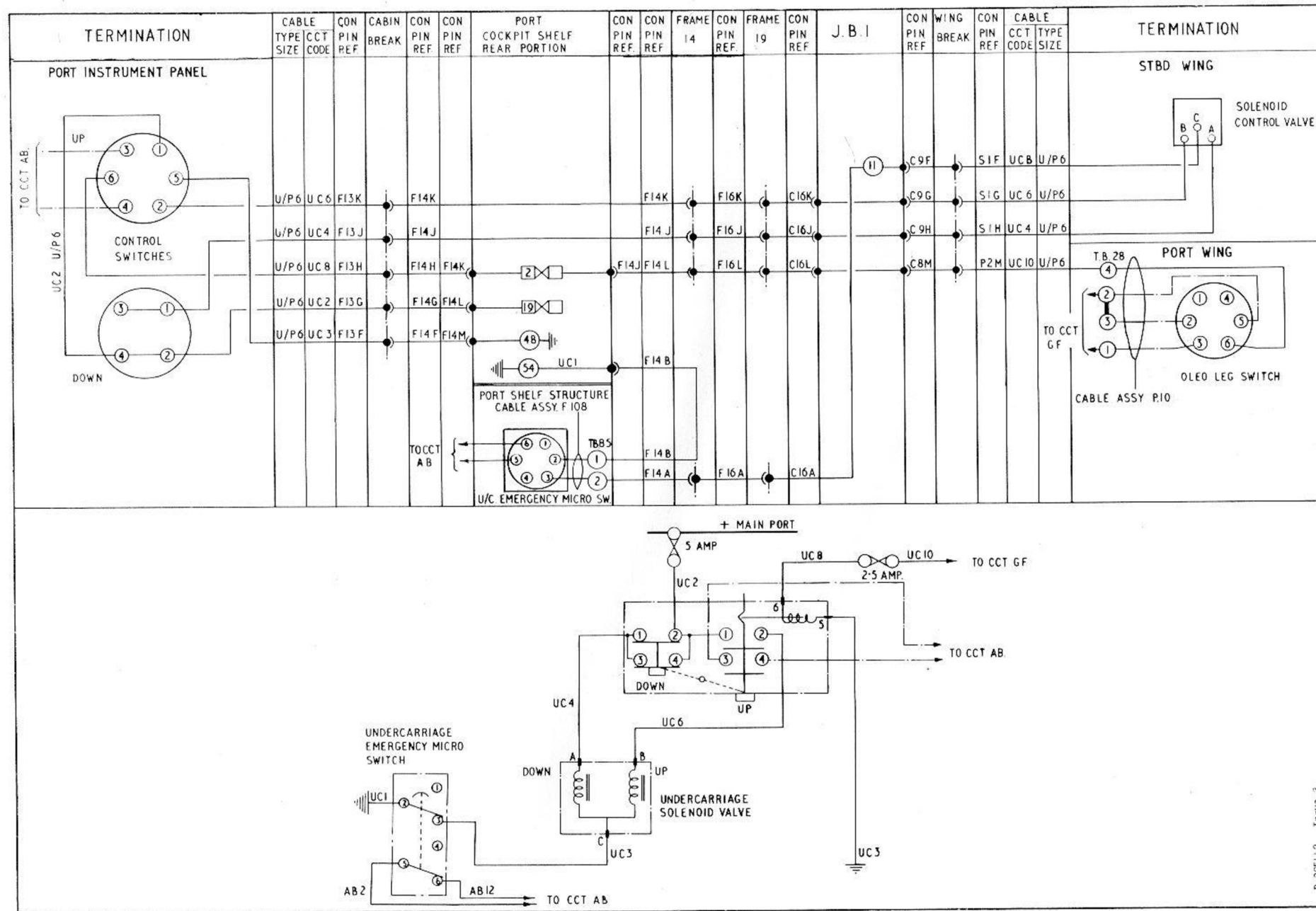
FIG. 1. ALIGHTING GEAR CONTROL
