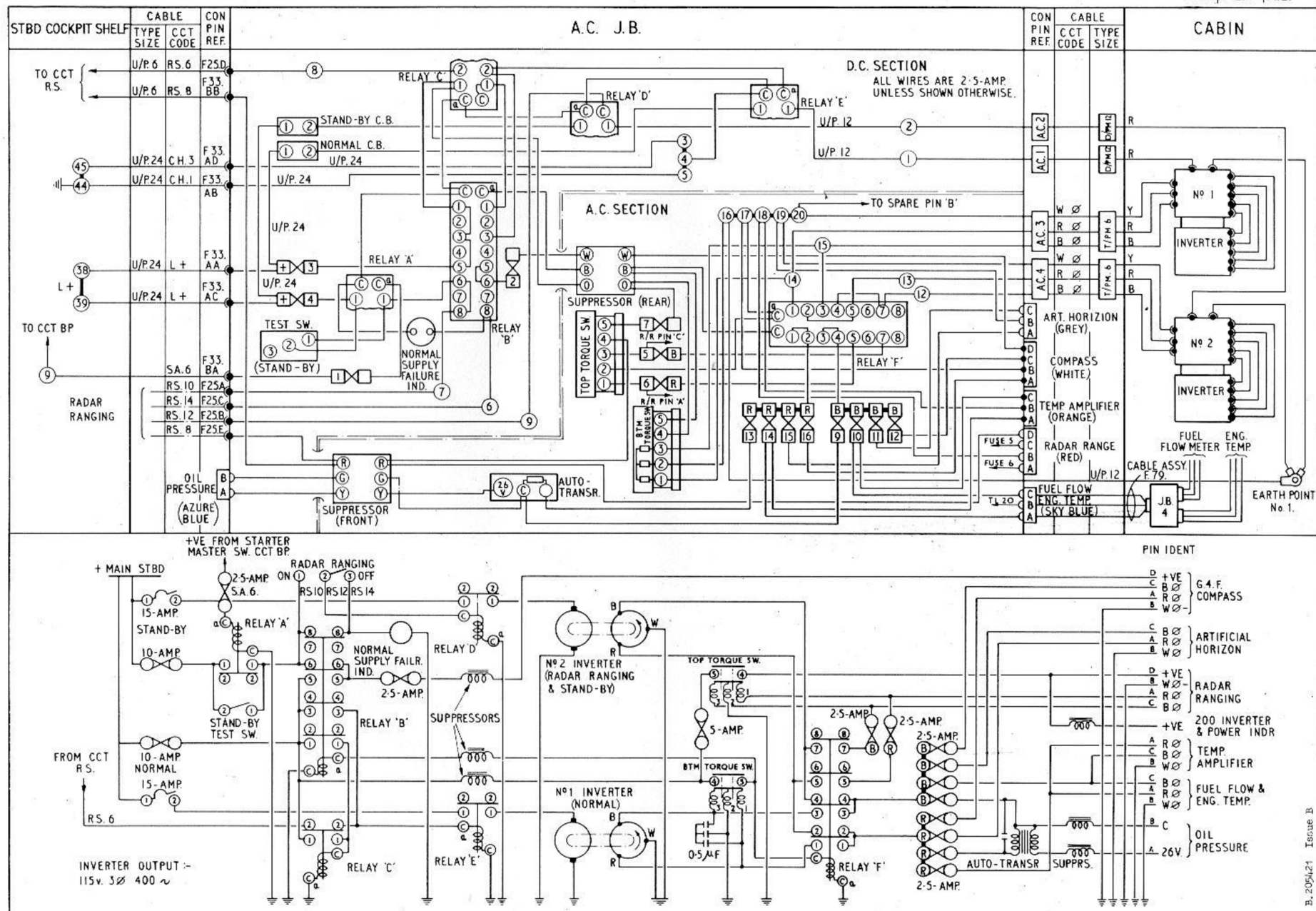
FIG. 1 A.C. SUPPLIES
