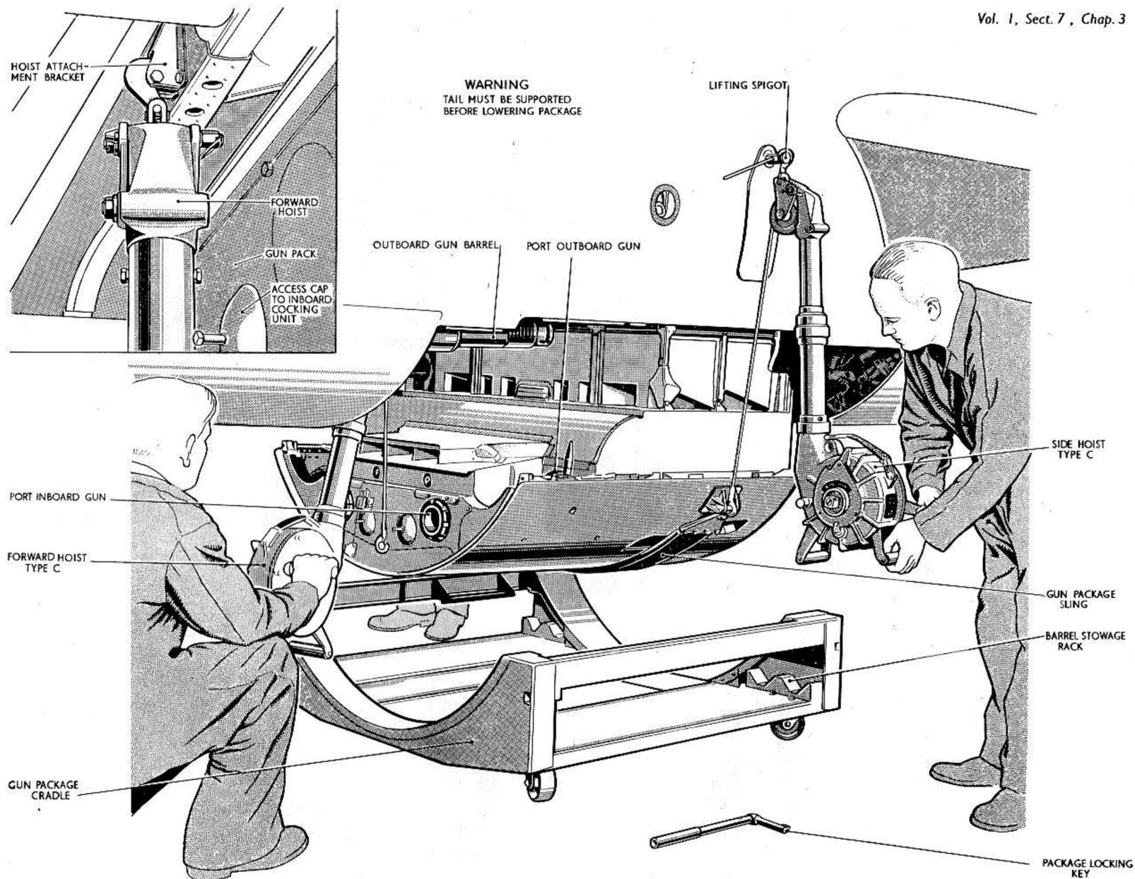
FIG. II PACKAGE REMOVAL (2)
