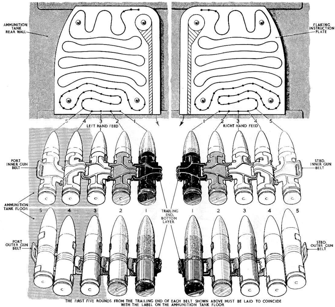
FIG.12 AMMUNITION FLAKING
