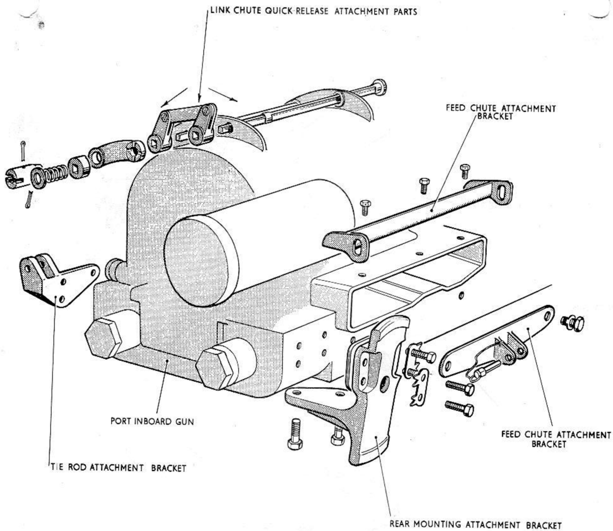
FIG.4 GUN FITTINGS
