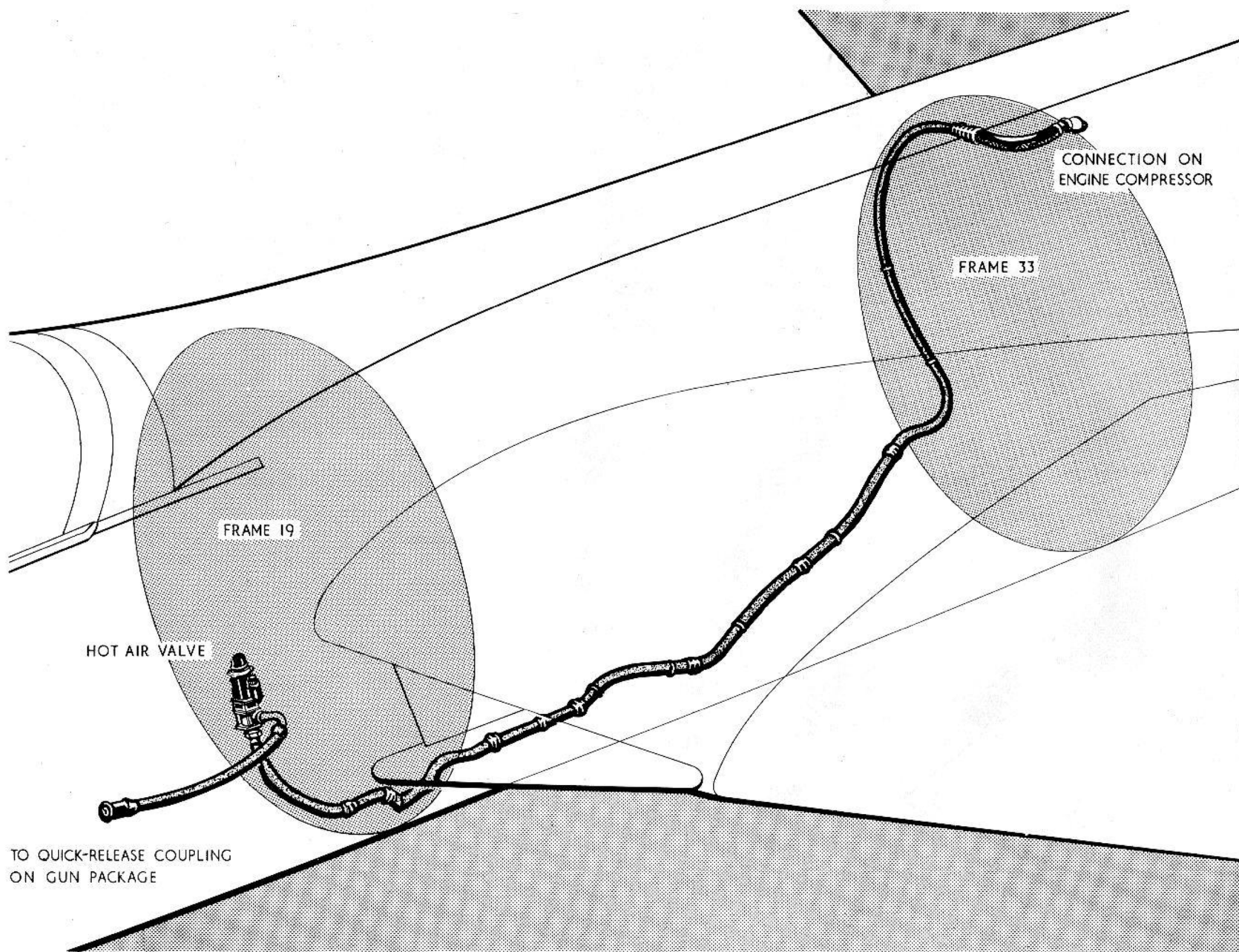
FIG.8-GUN HEATING INSTALLATION
