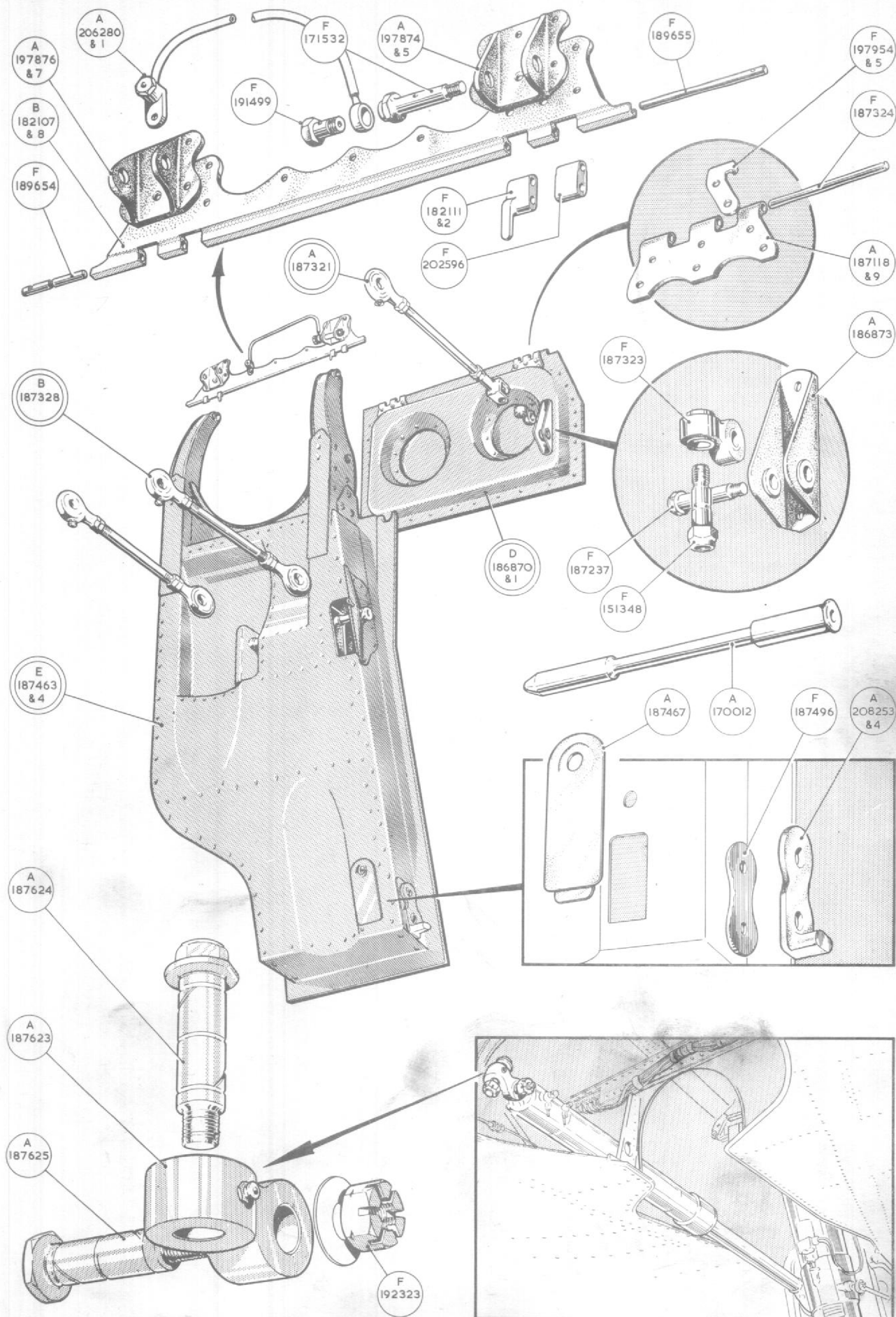
MAIN UNDERCARRIAGE
