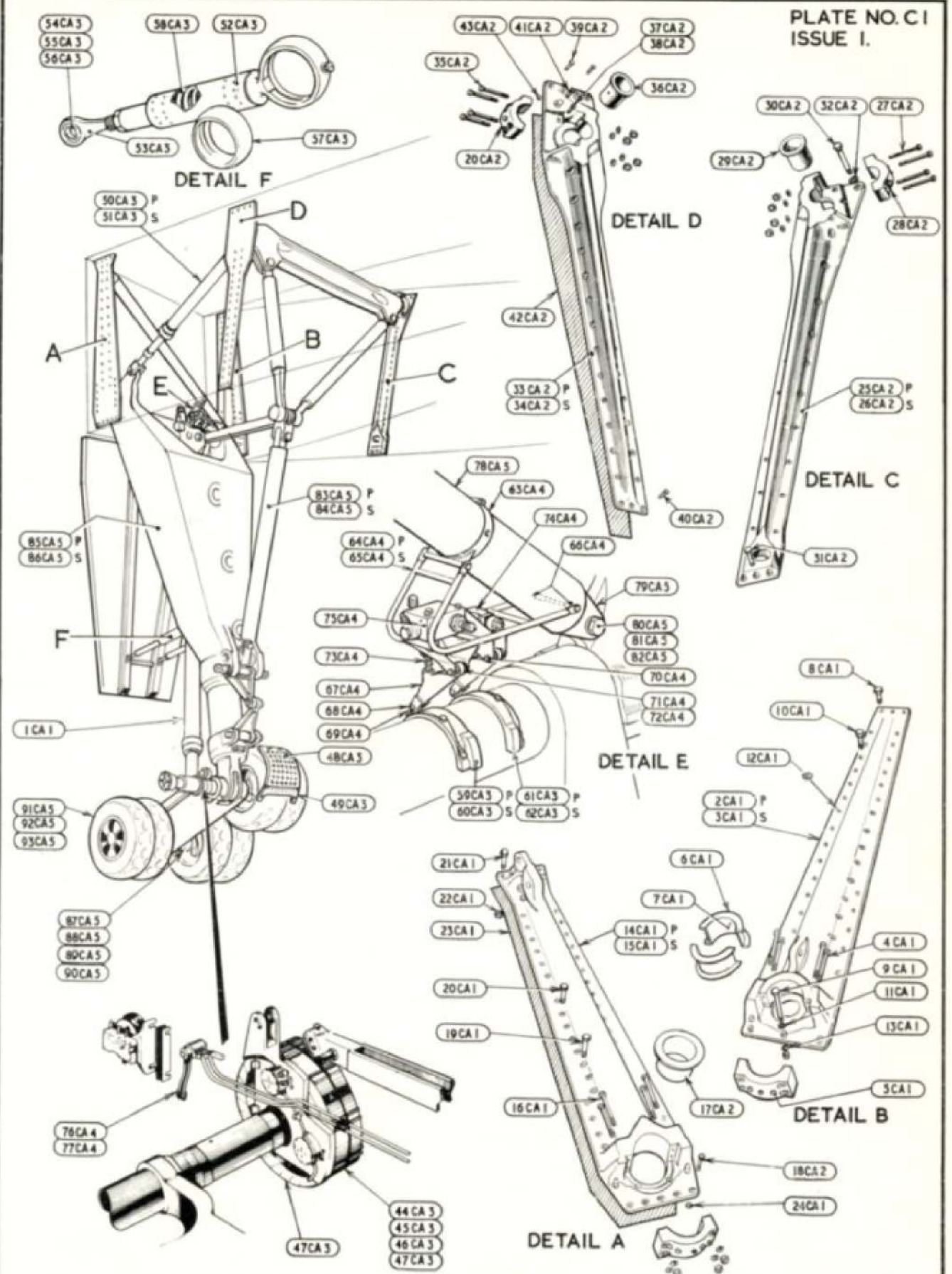
ALIGHTING GEAR - MAIN UNDERCARRIAGE
