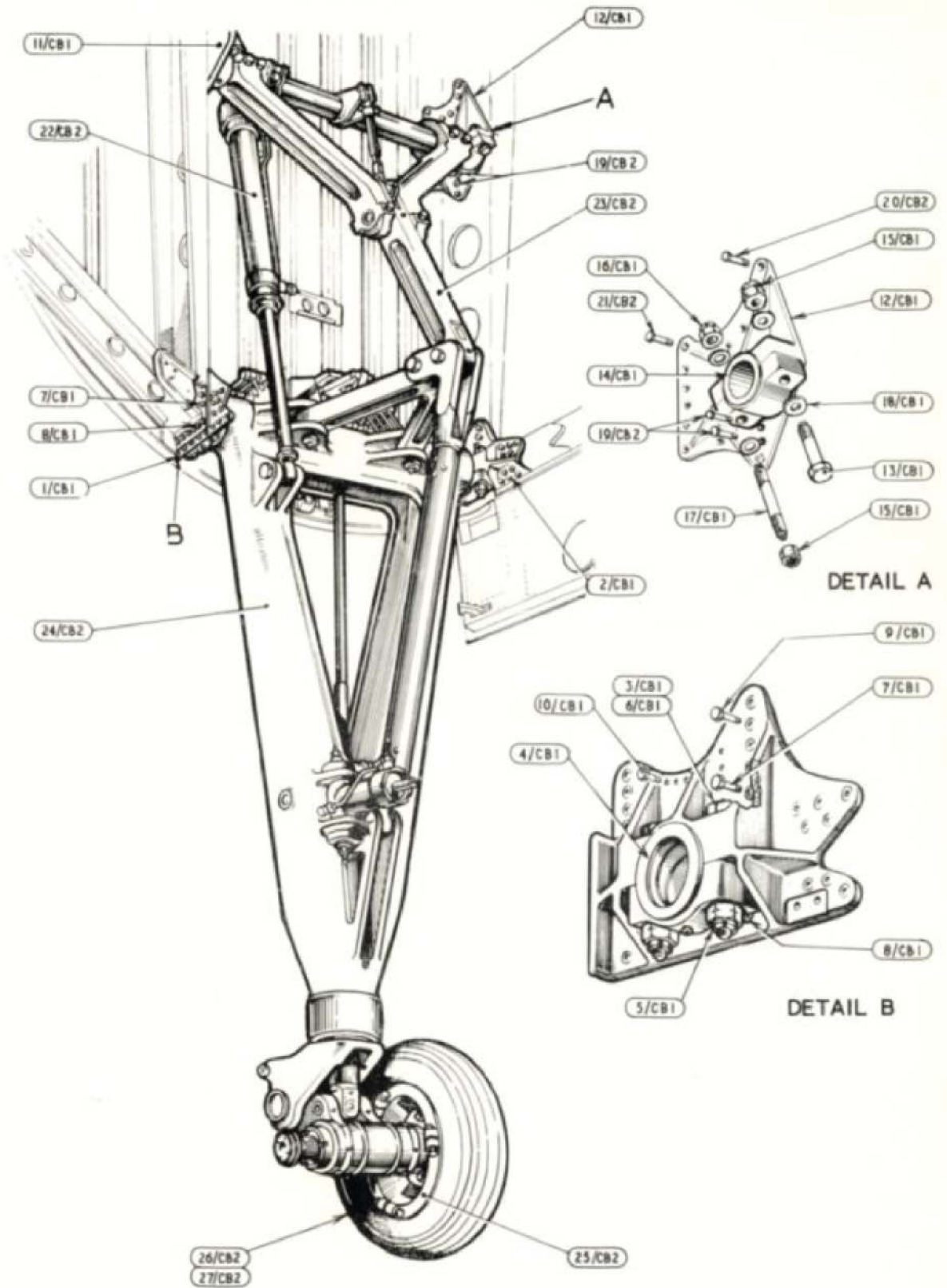
ALIGHTING GEAR — NOSEWHEEL UNDERCARRIAGE
