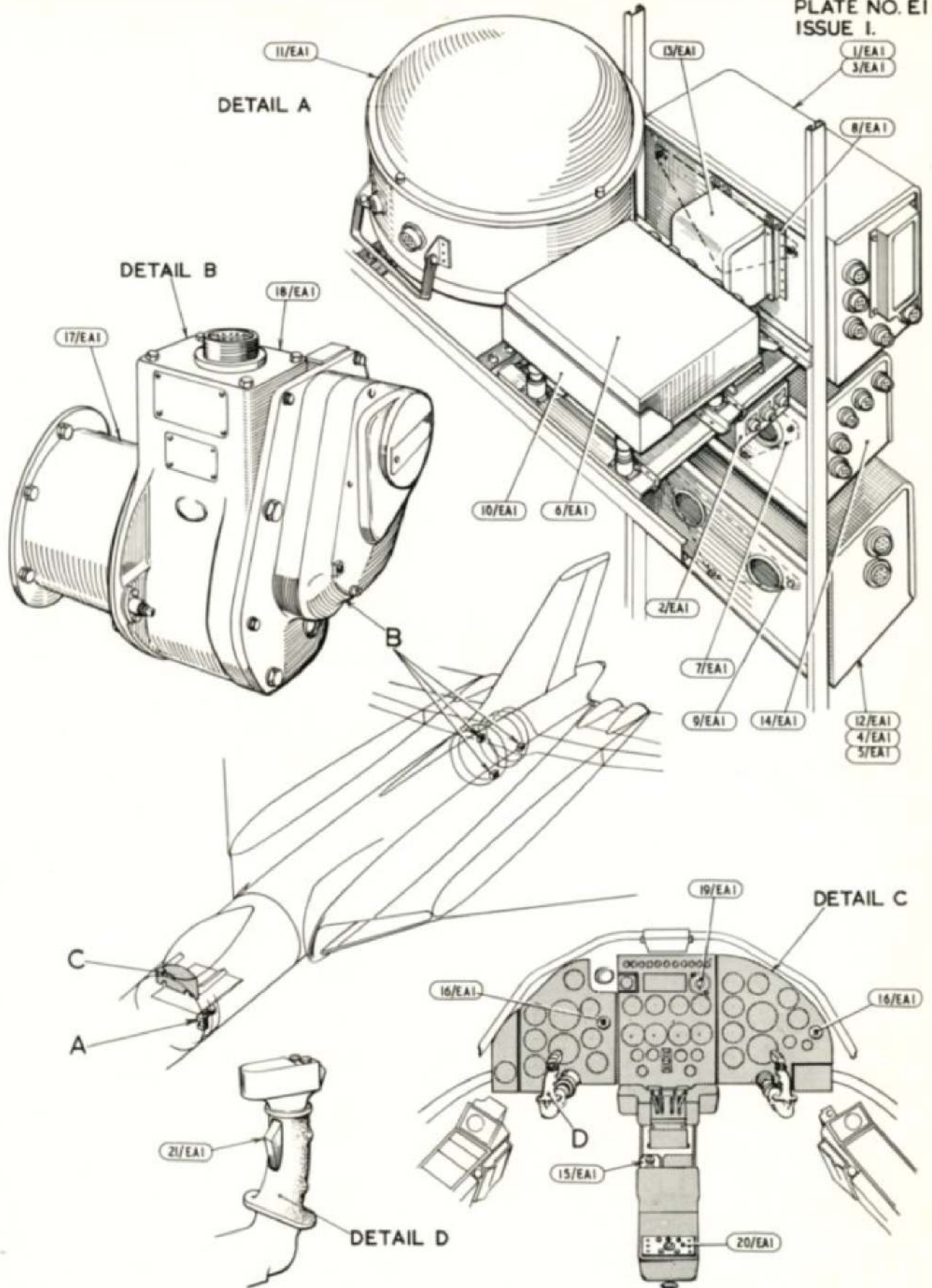
AUTO-PILOT CONTROLS
