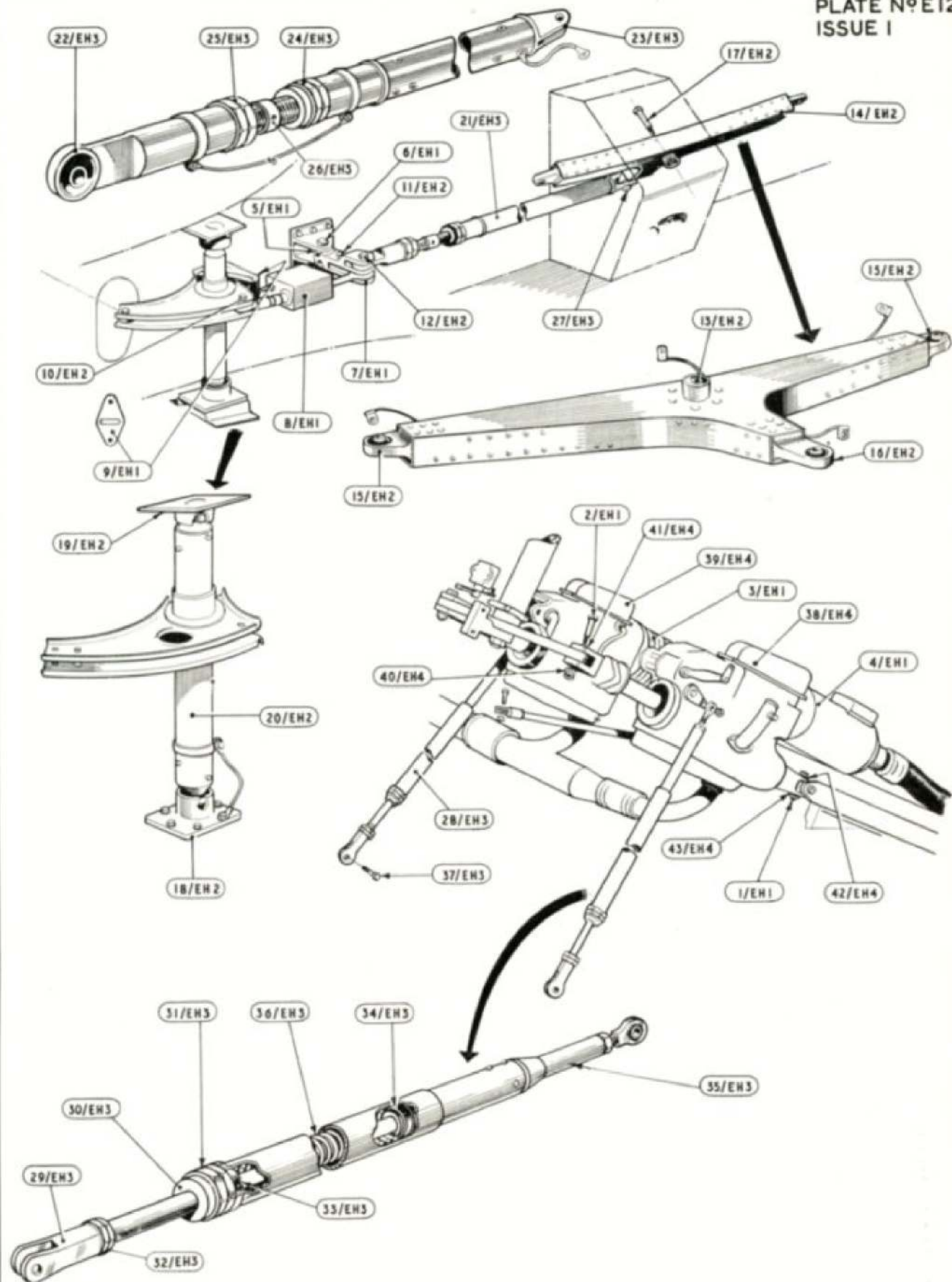
FLYING CONTROLS REAR PORTION FUSELAGE
