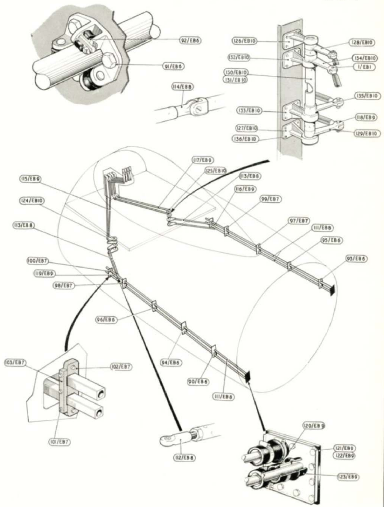
ENGINE CONTROLS CREWS NACELLE (1)
