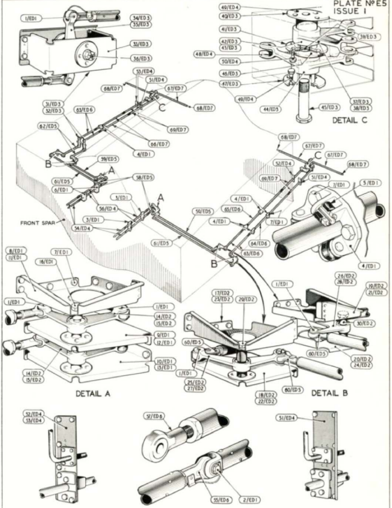
ENGINE CONTROLS - AFT OF FRONT SPAR CENTRE PORTION FUSELAGE
