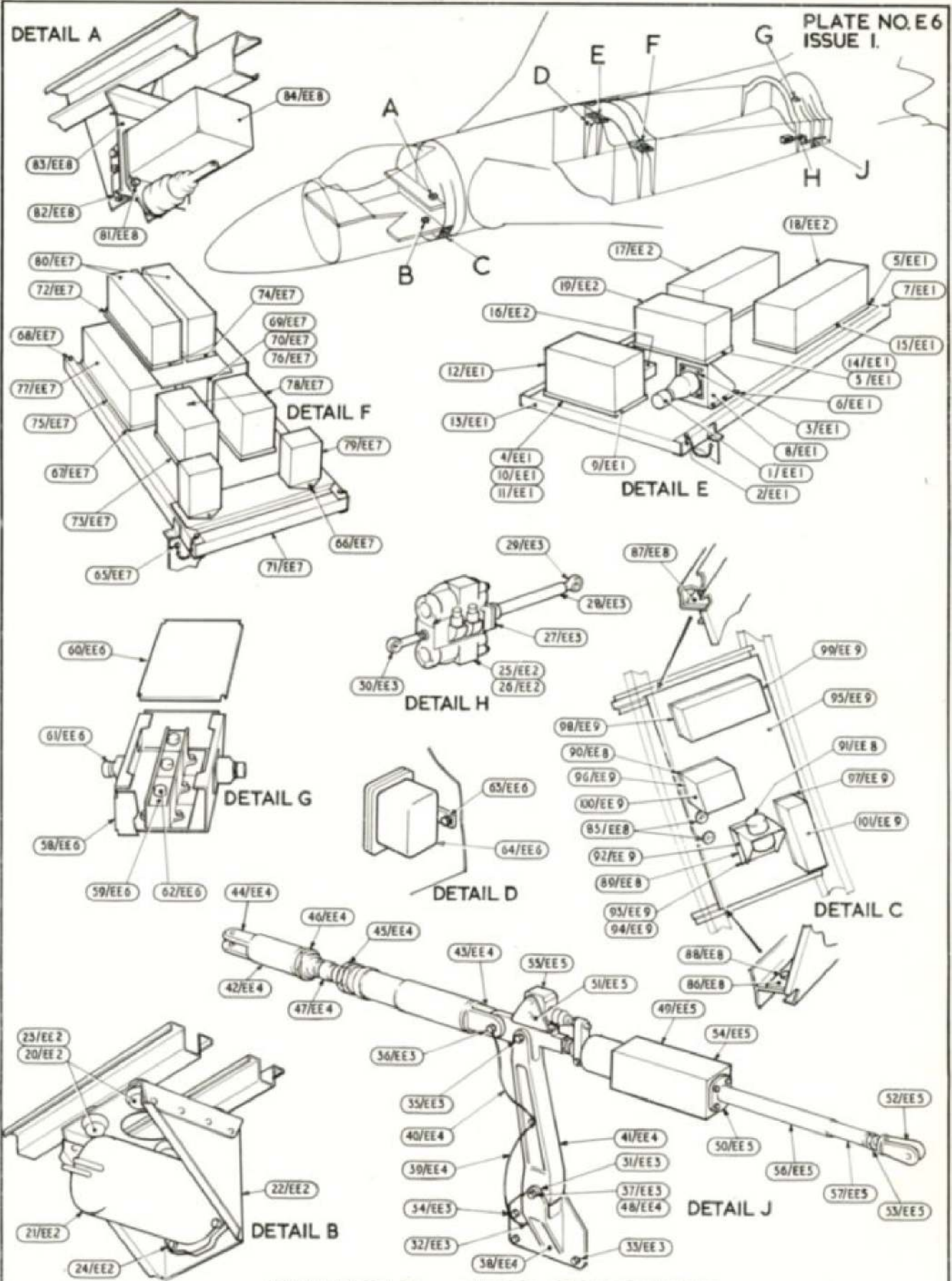
CONTROLS — AUTO STABILISER
