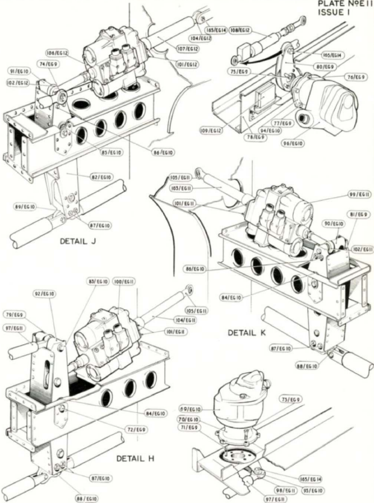
FLYING CONTROLS IN CENTRE PORTION FUSELAGE (3)
