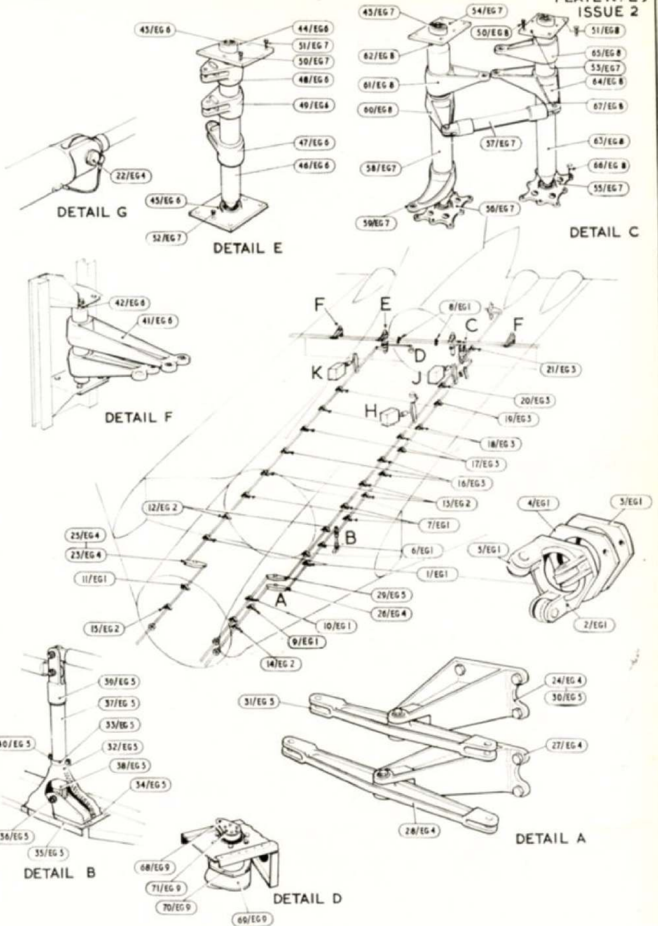
FLYING CONTROLS IN CENTRE PORTION FUSELAGE (1)
