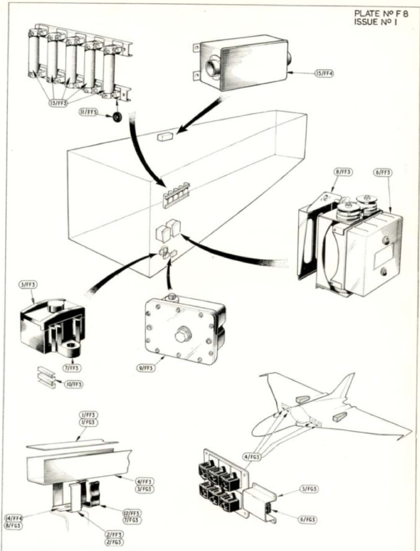
ELECTRICAL INSTALLATION — CENTRE PORTION COMPARTMENTS AFT OF UNDERCARRIAGE BAYS. UNDER AIR INTAKES.
