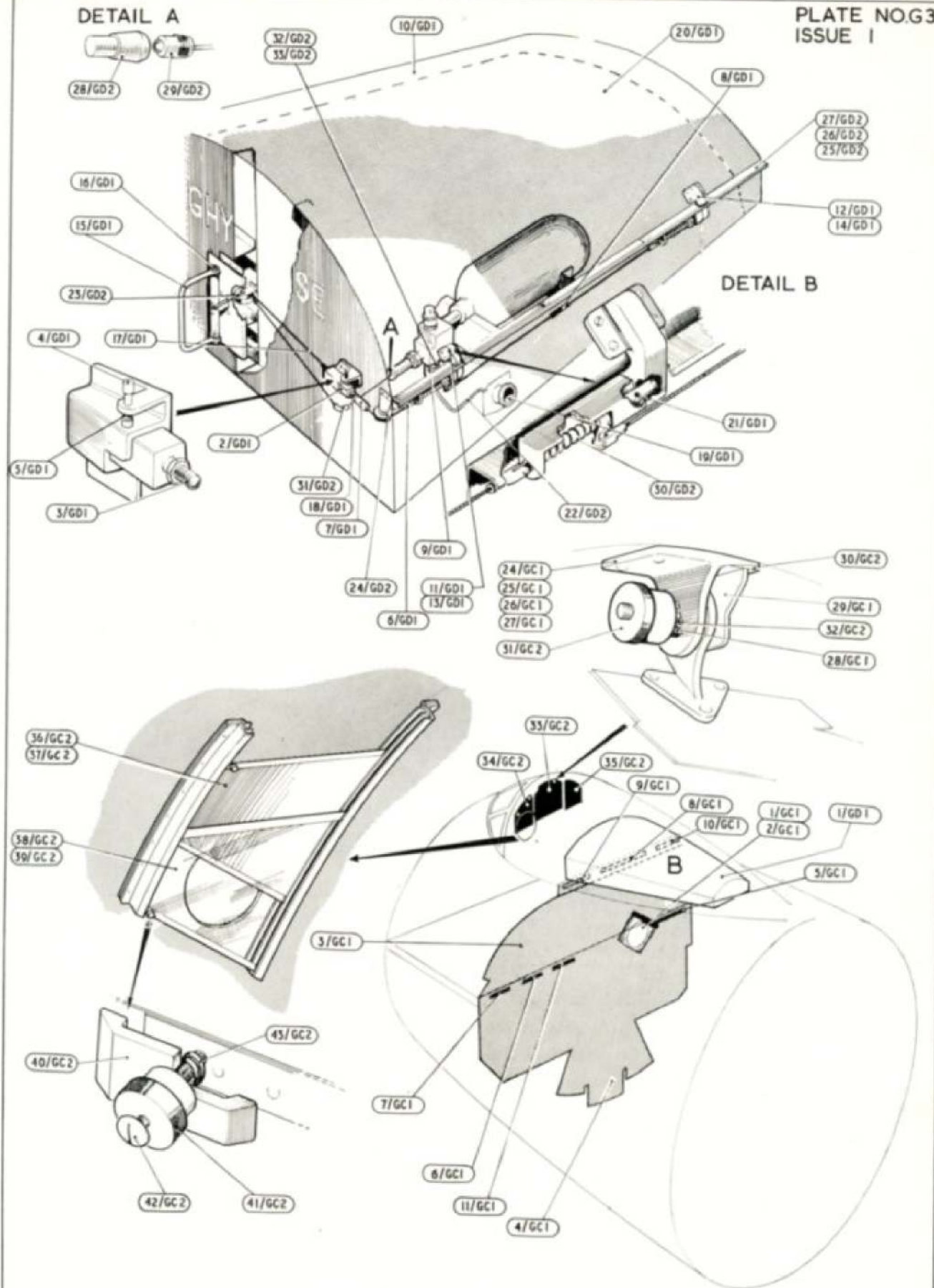
AIRCRAFT EQUIPMENT DINGHY INSTALLATION - CURTAINS & VISORS
