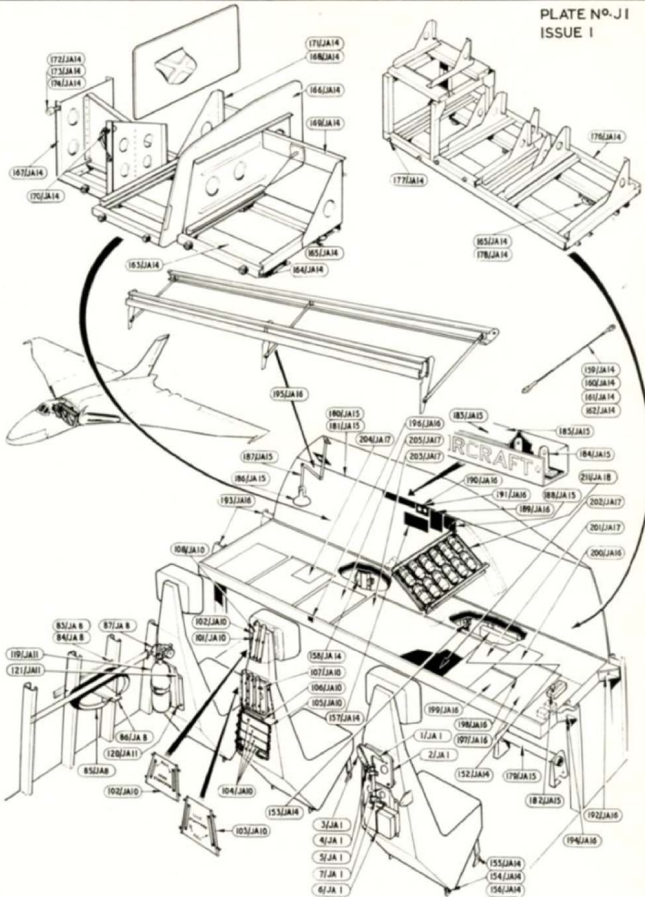
FUSELAGE CREW'S NACELLE (I)
