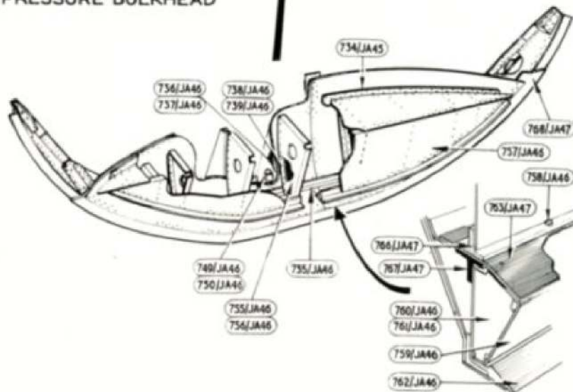
FORWARD PRESSURE BULKHEAD
