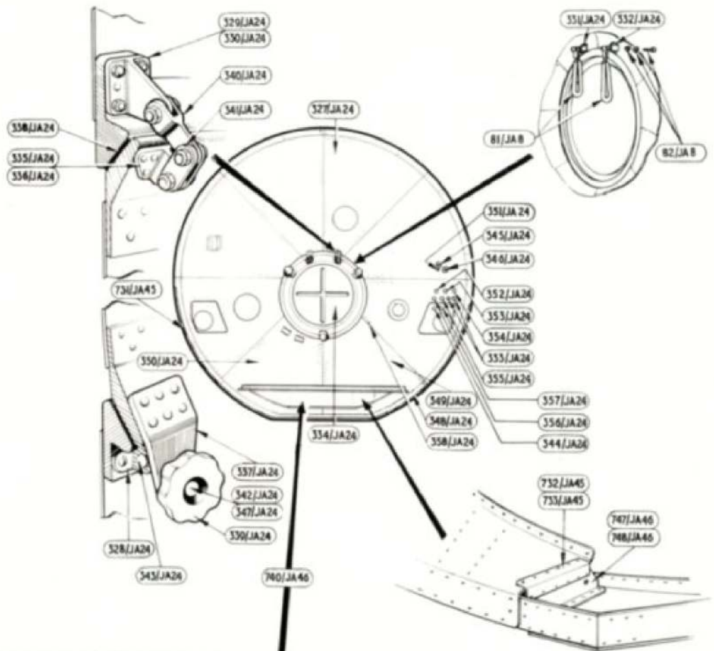
FORWARD PRESSURE BULKHEAD
