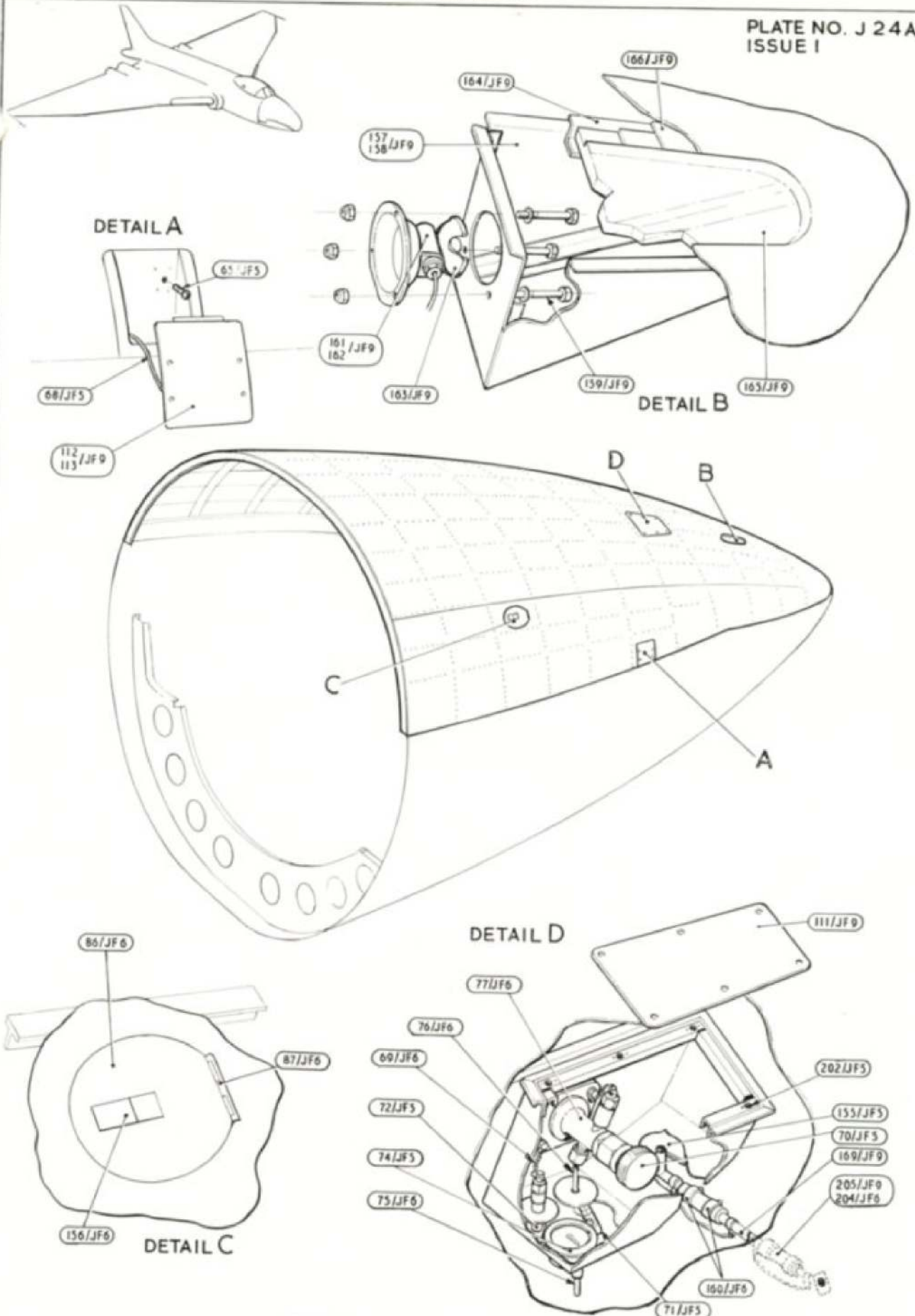
FUSELAGE-NOSE PORTION (3)
