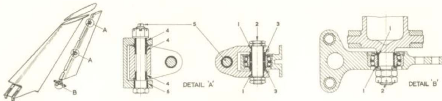
Fig.401. Rudder hinges
