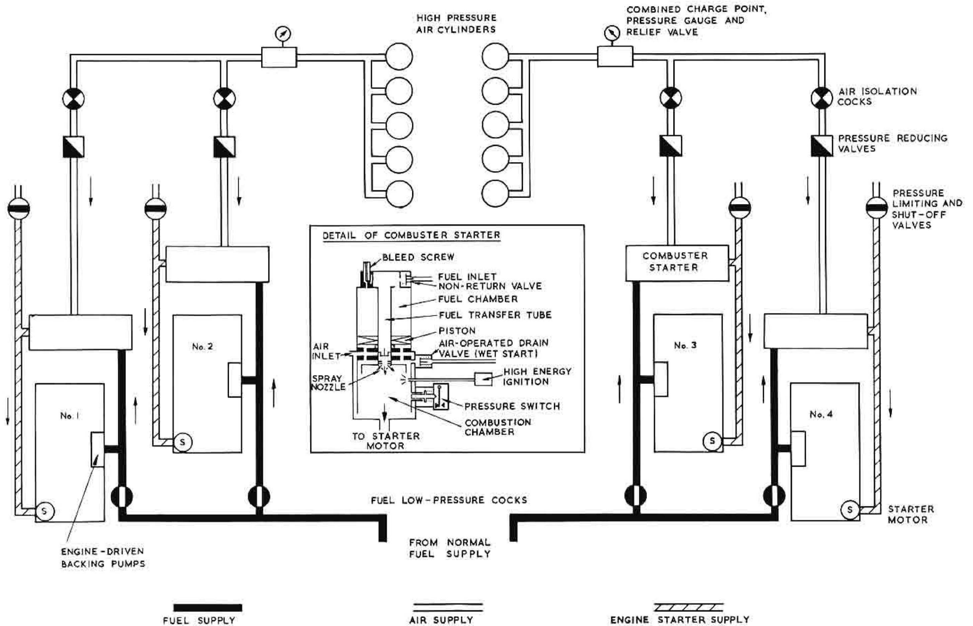
Fig. 2 Rapid start system
