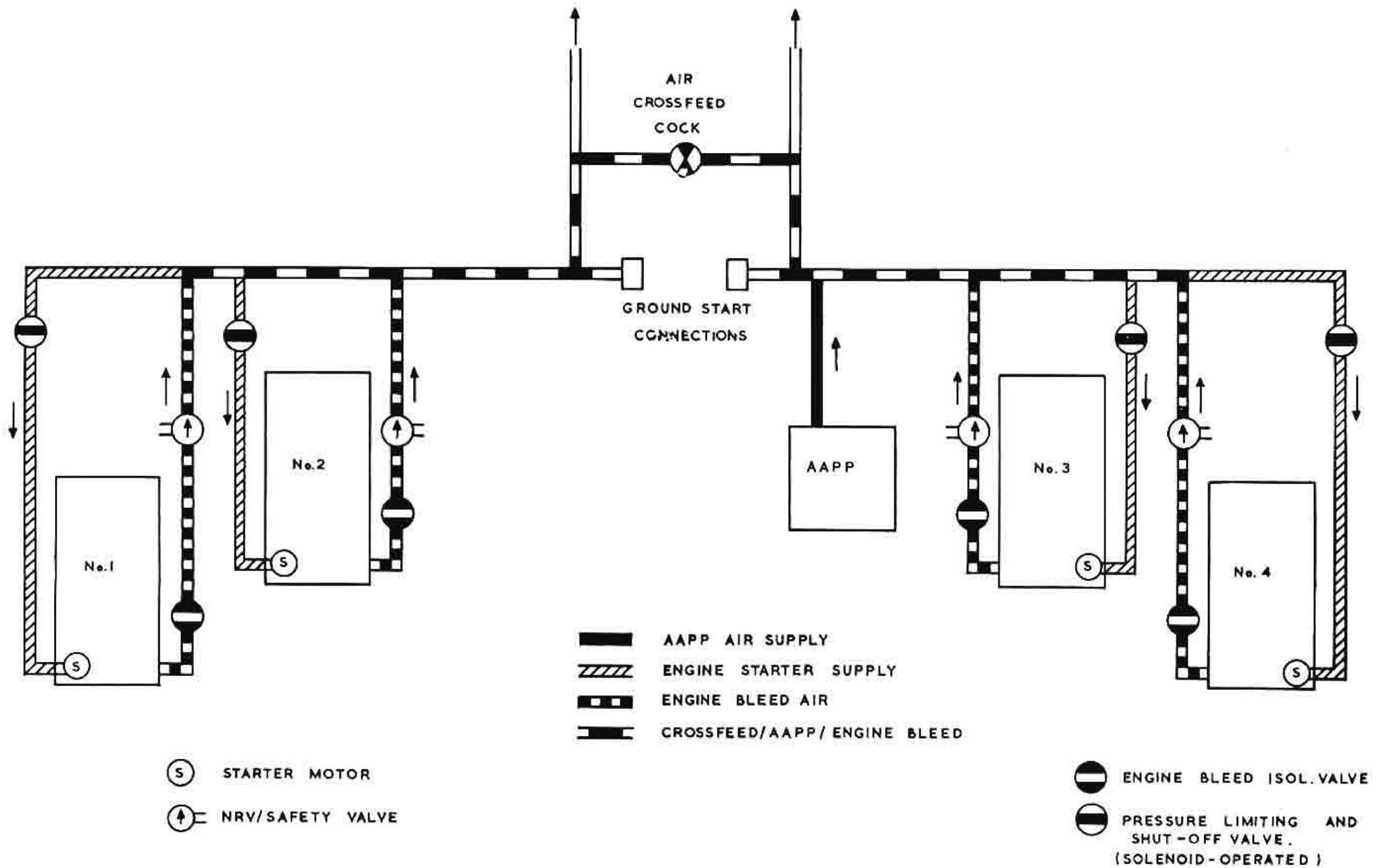
Fig. 1 Normal engine starting system
