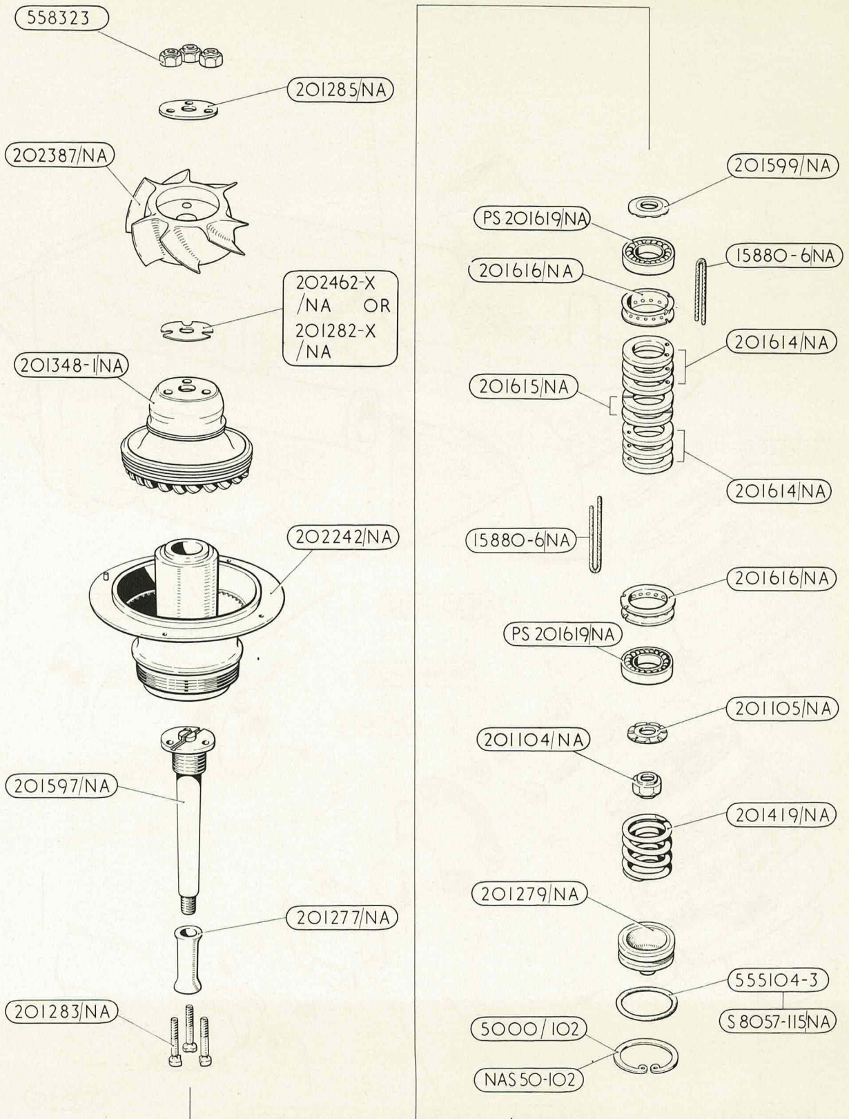
ROTATING ASSEMBLY.
