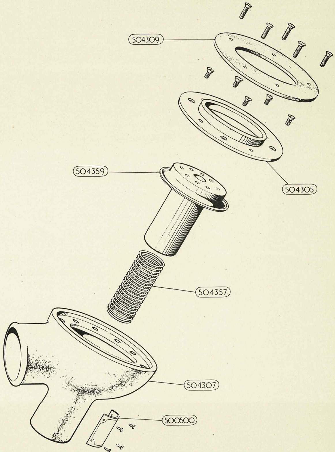
COUPLING, RADAR COOLING
