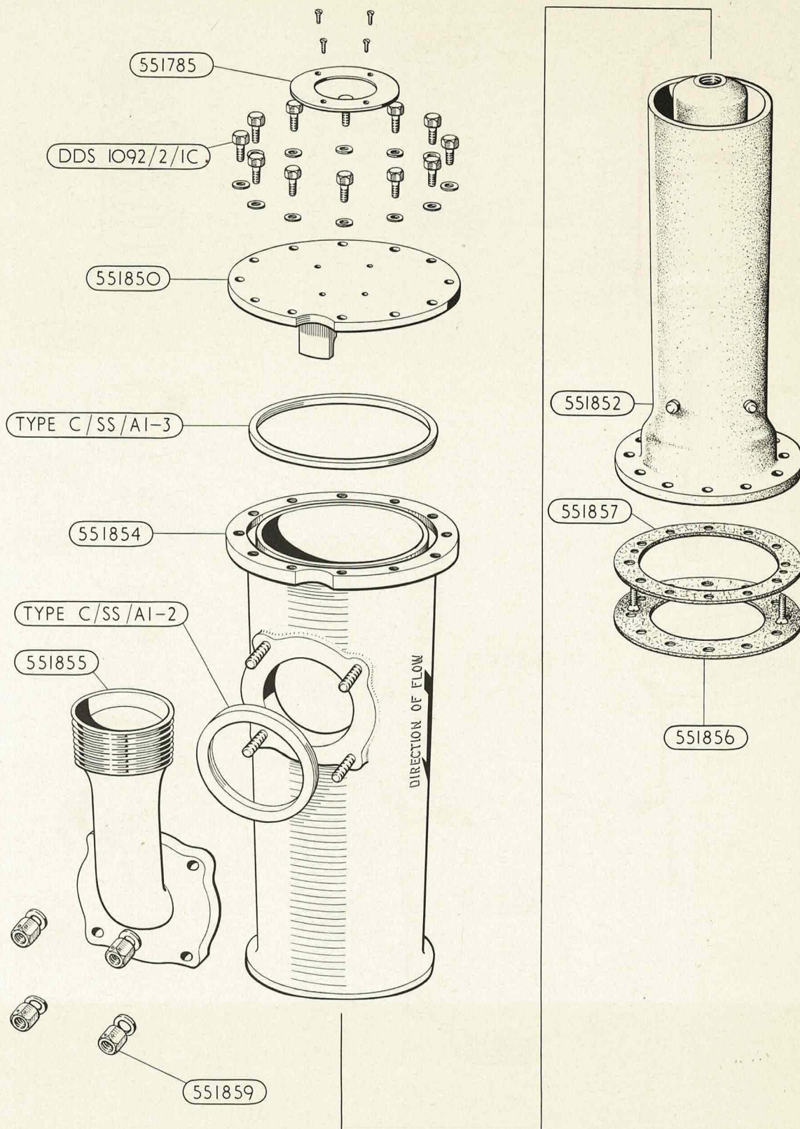
VALVE, CONSTANT FLOW
