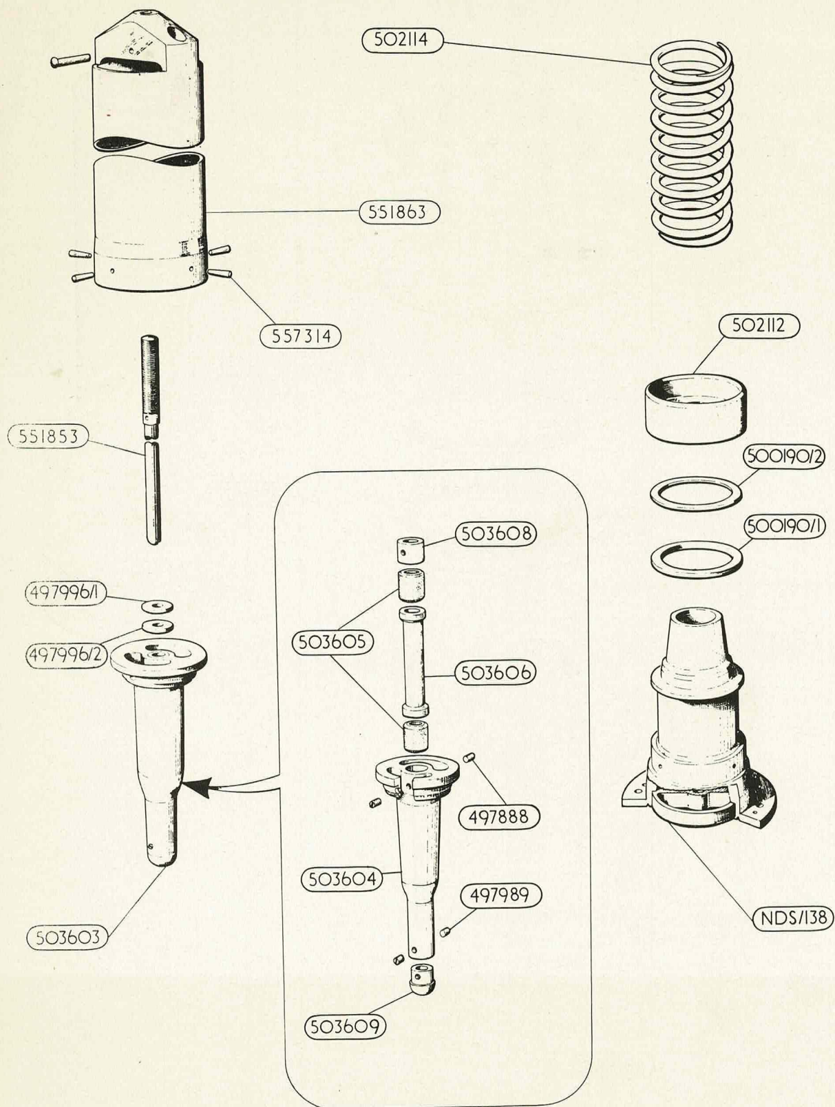
ORIFICE &amp; FLOW CONTROLLER ASSEMBLY
