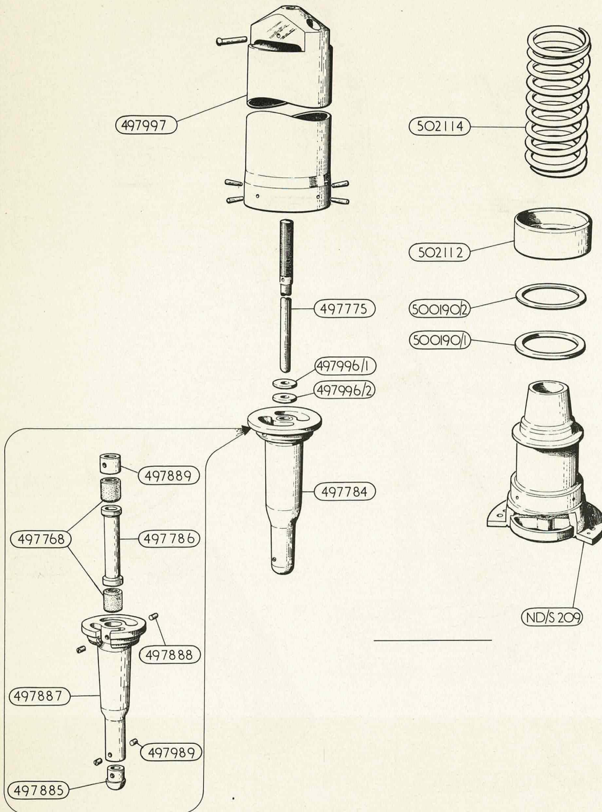
ORIFICE AND FLOW CONTROLLER ASSEMBLY
