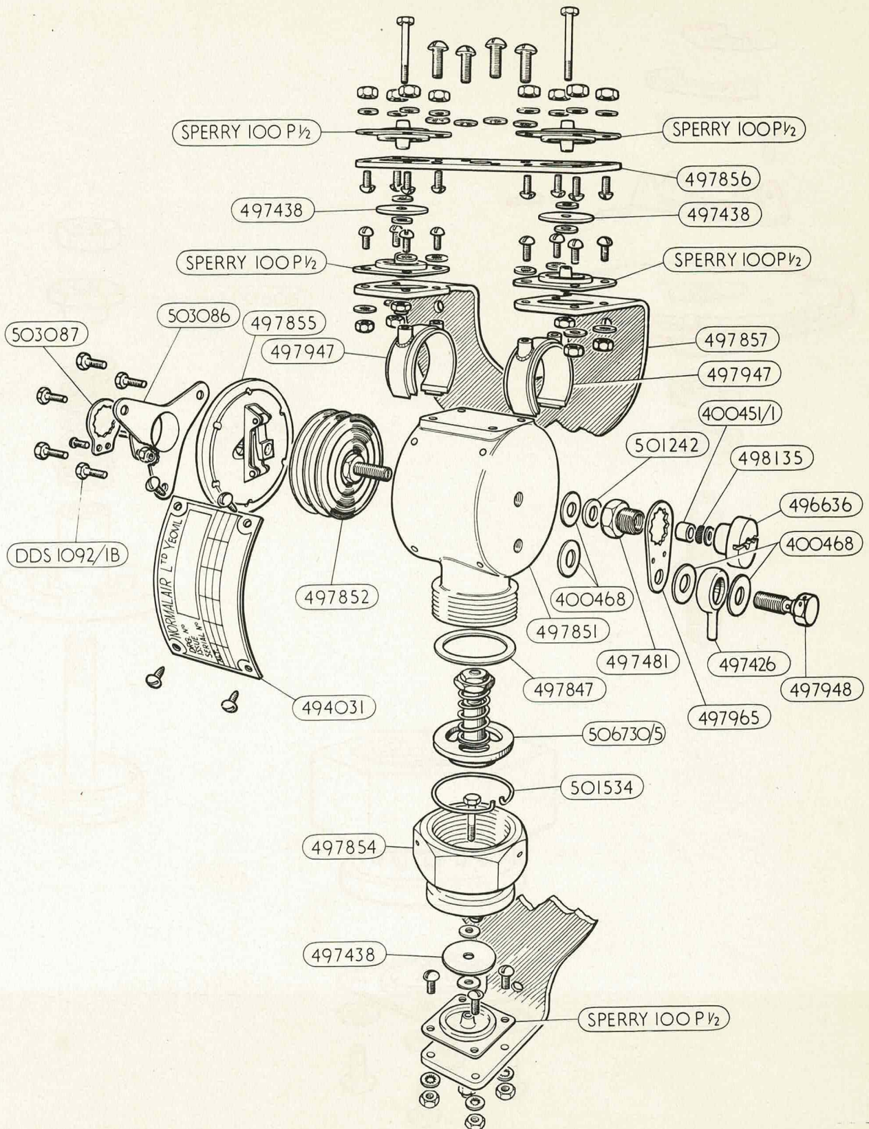
VALVE , REDUCING
