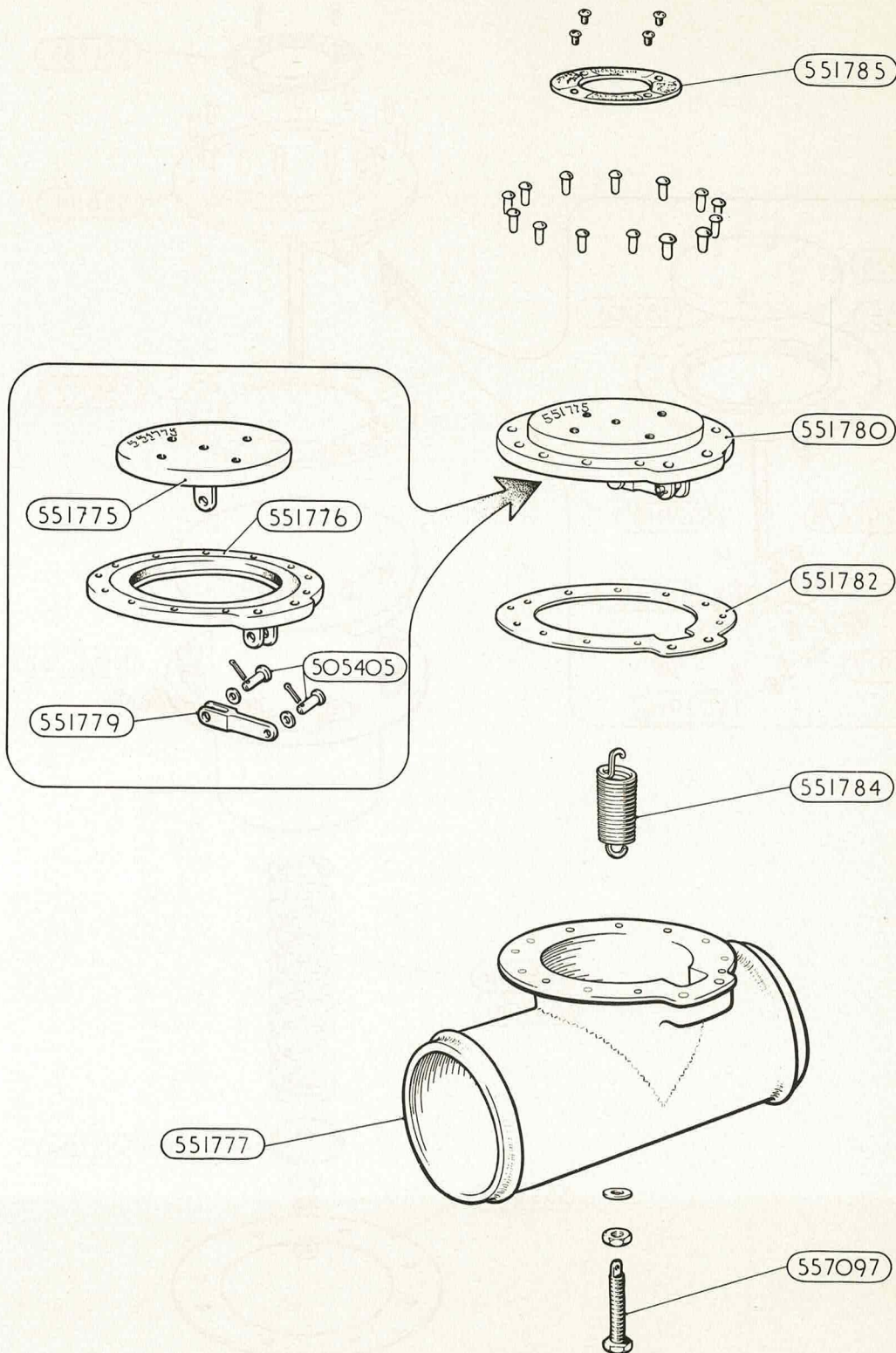
VALVE, RELIEF
