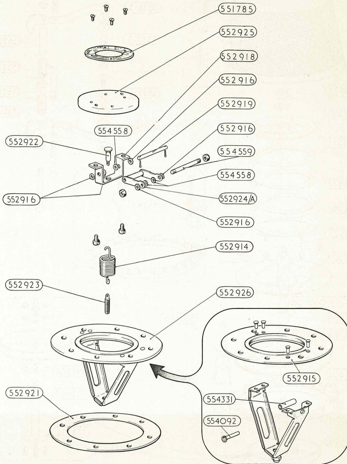
RELIEF VALVE
