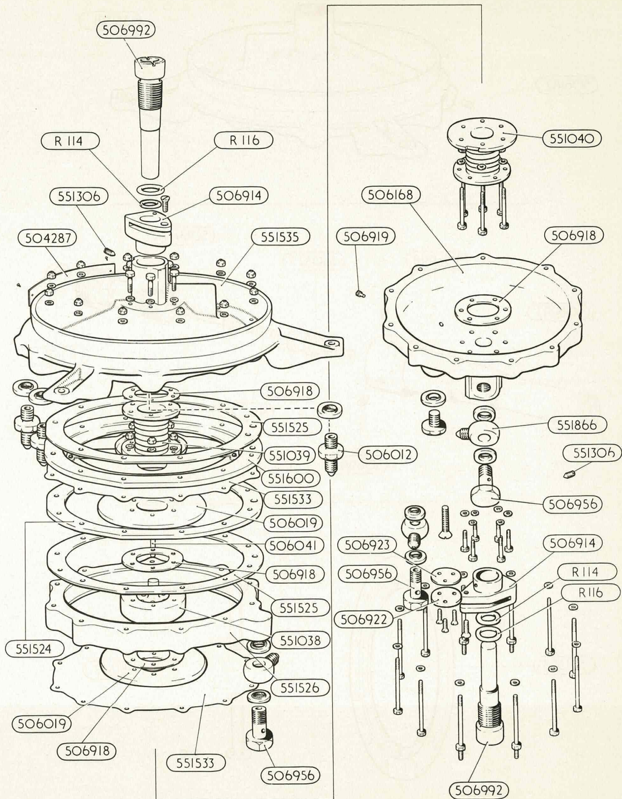
VALVE, RELAY
