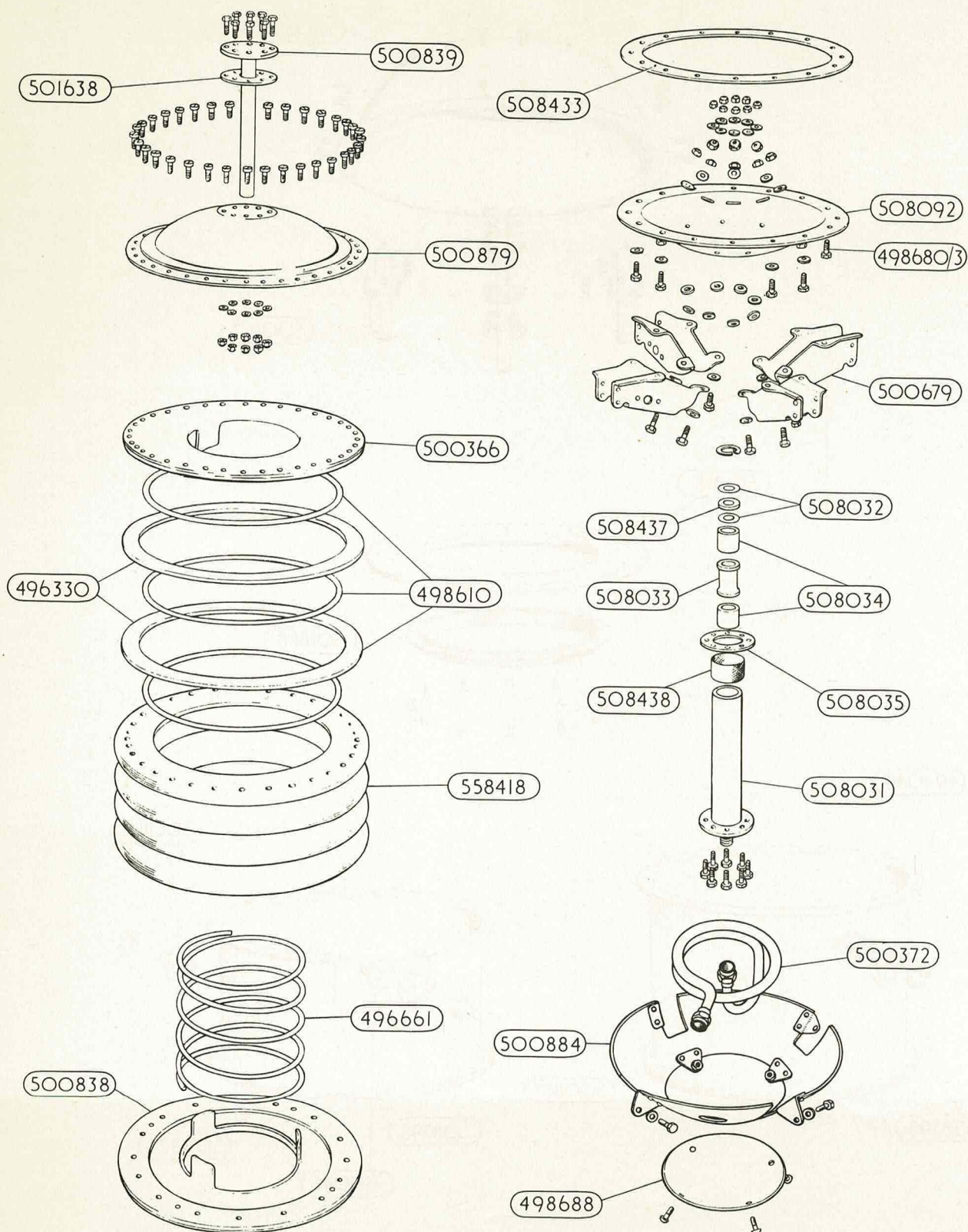
DIAPHRAGM, UPPER ASSEMBLY
