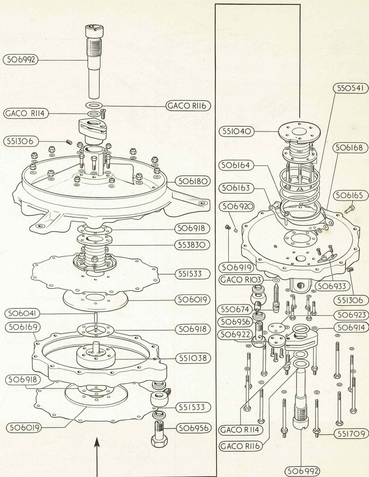
CONTROLLER, SURGE, ASSEMBLY
