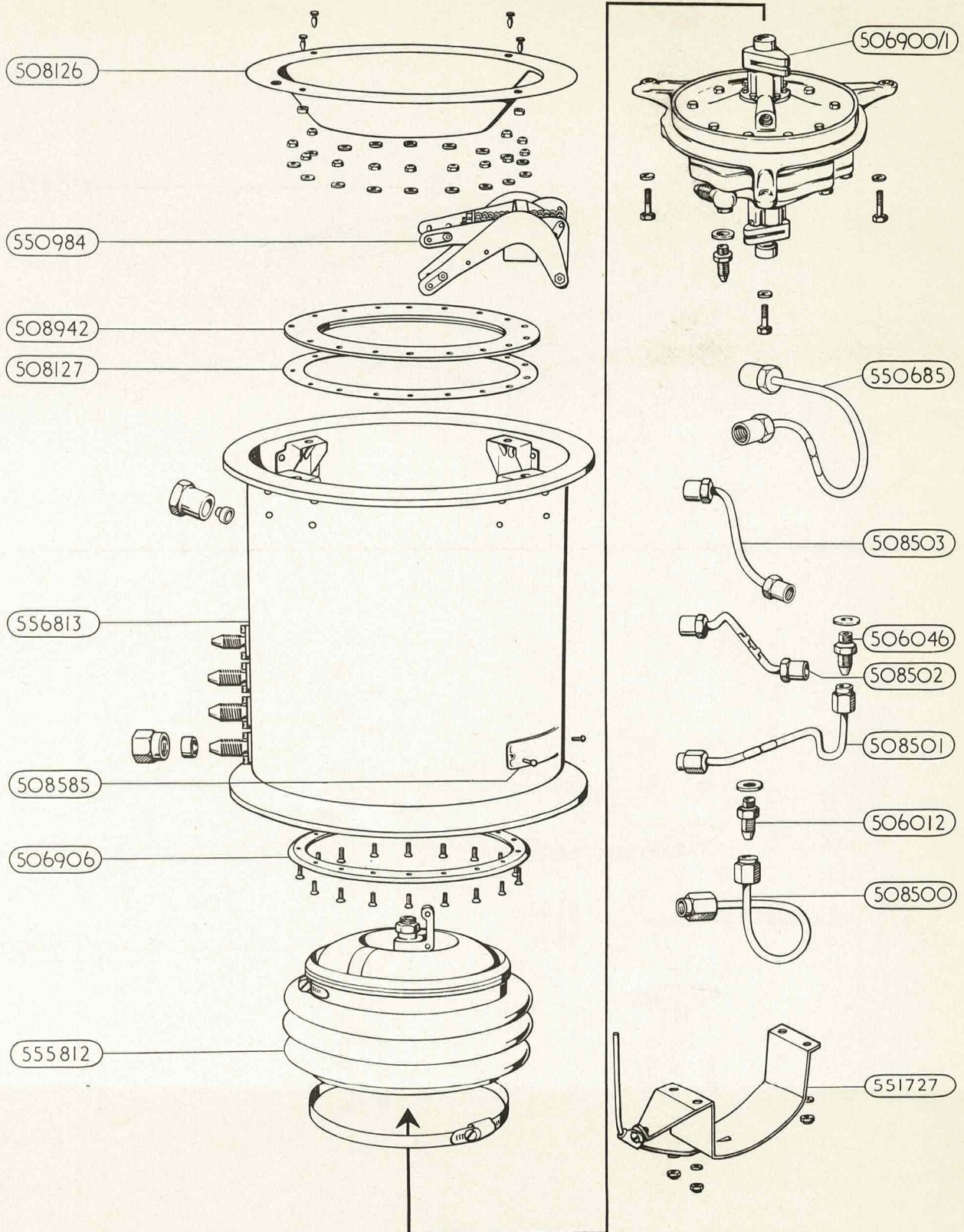
UNIT, No.2. ASSEMBLY.
