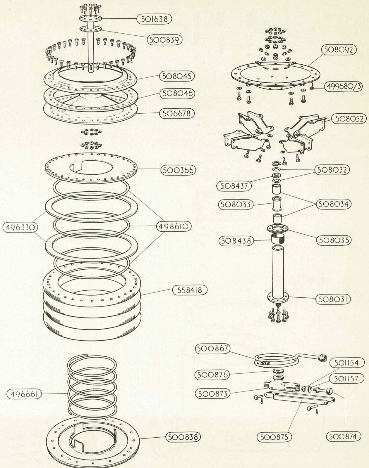
DIAPHRAGM, LOWER ASSEMBLY
