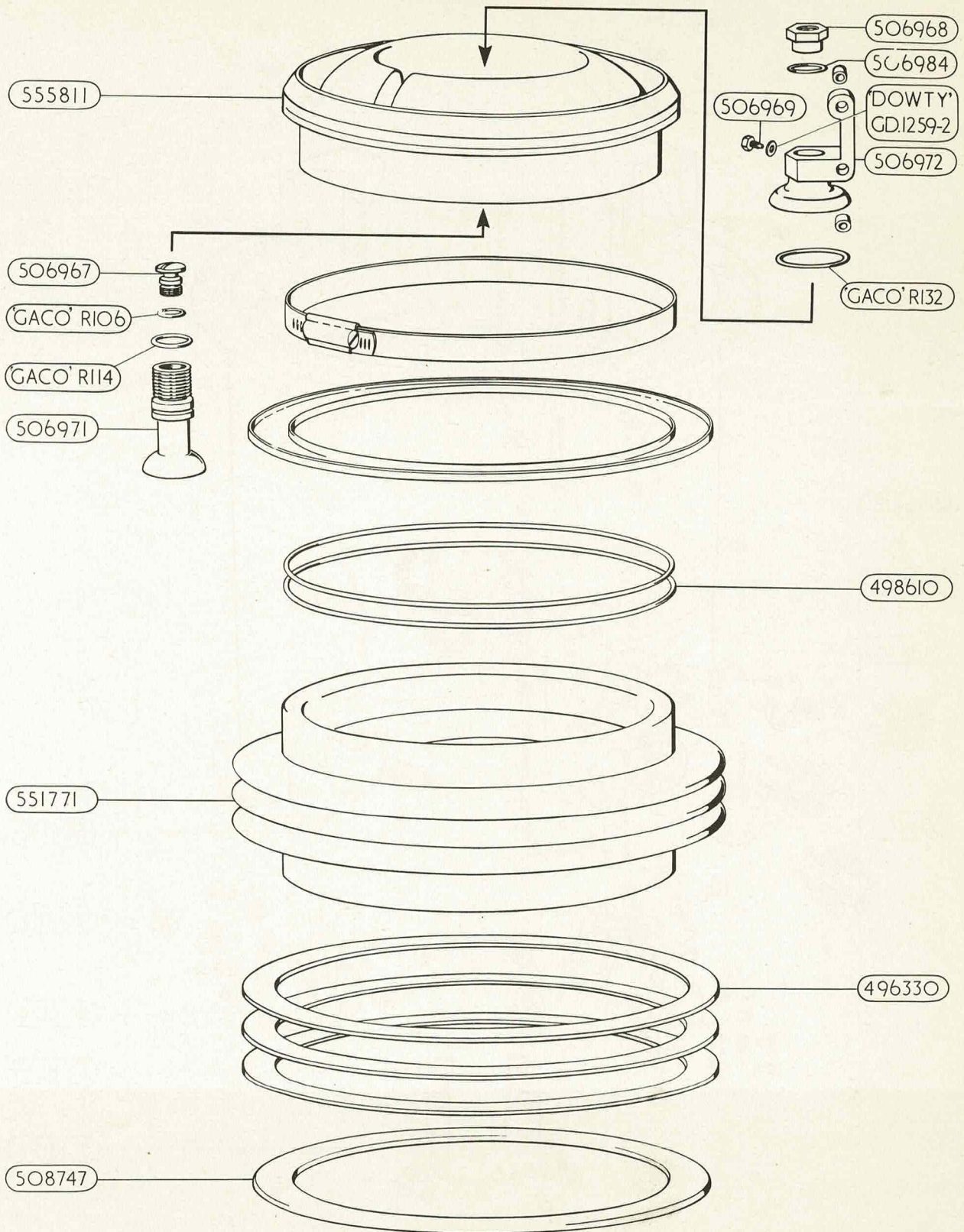
BELLOWS ASSEMBLY
