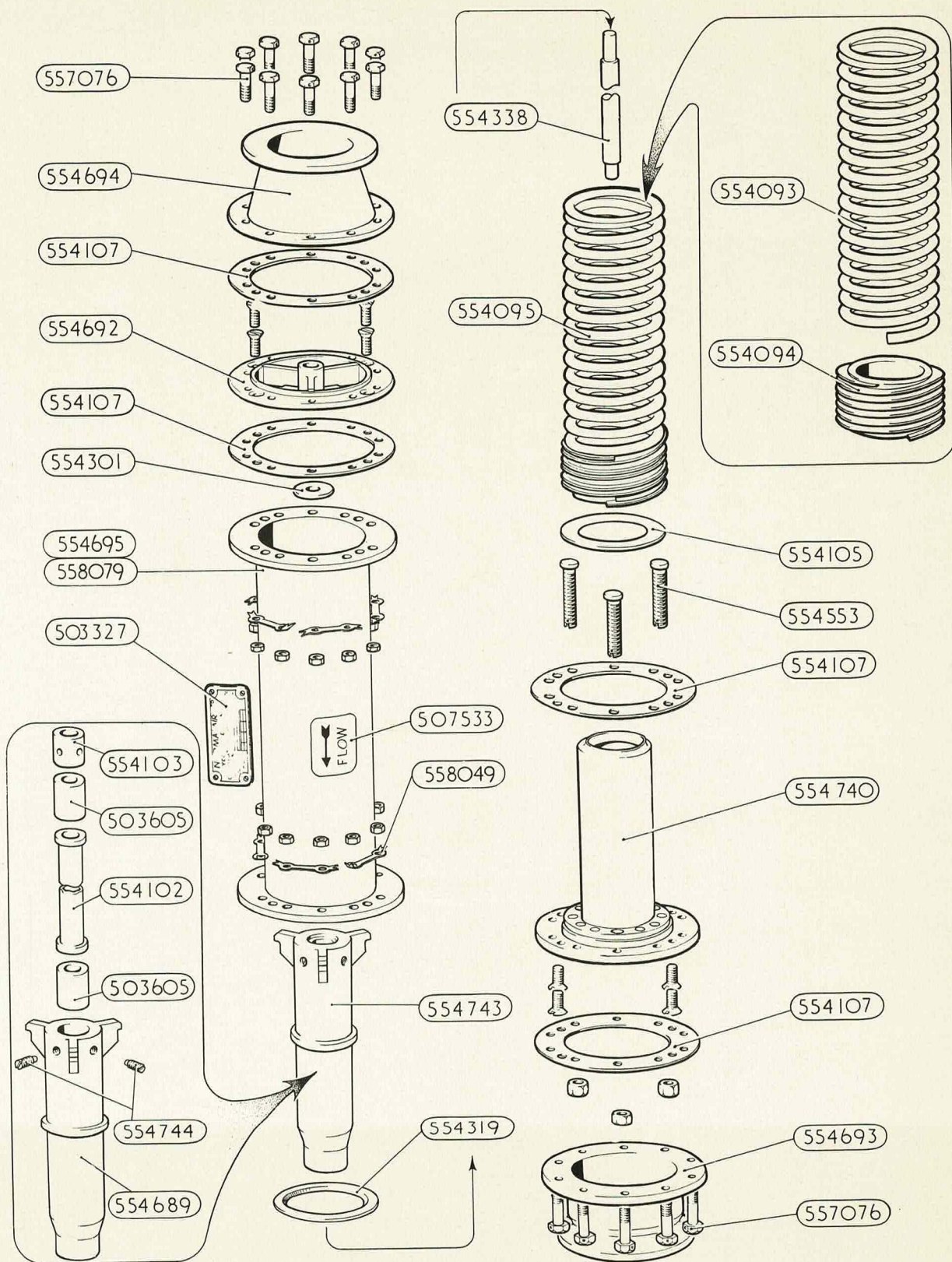
AUGMENTOR, FLOW
