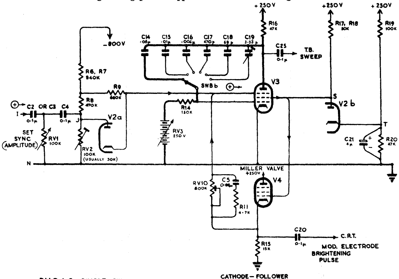
DIAG. 1.2 SINGLE SWEEP T.B.-GENERATOR
